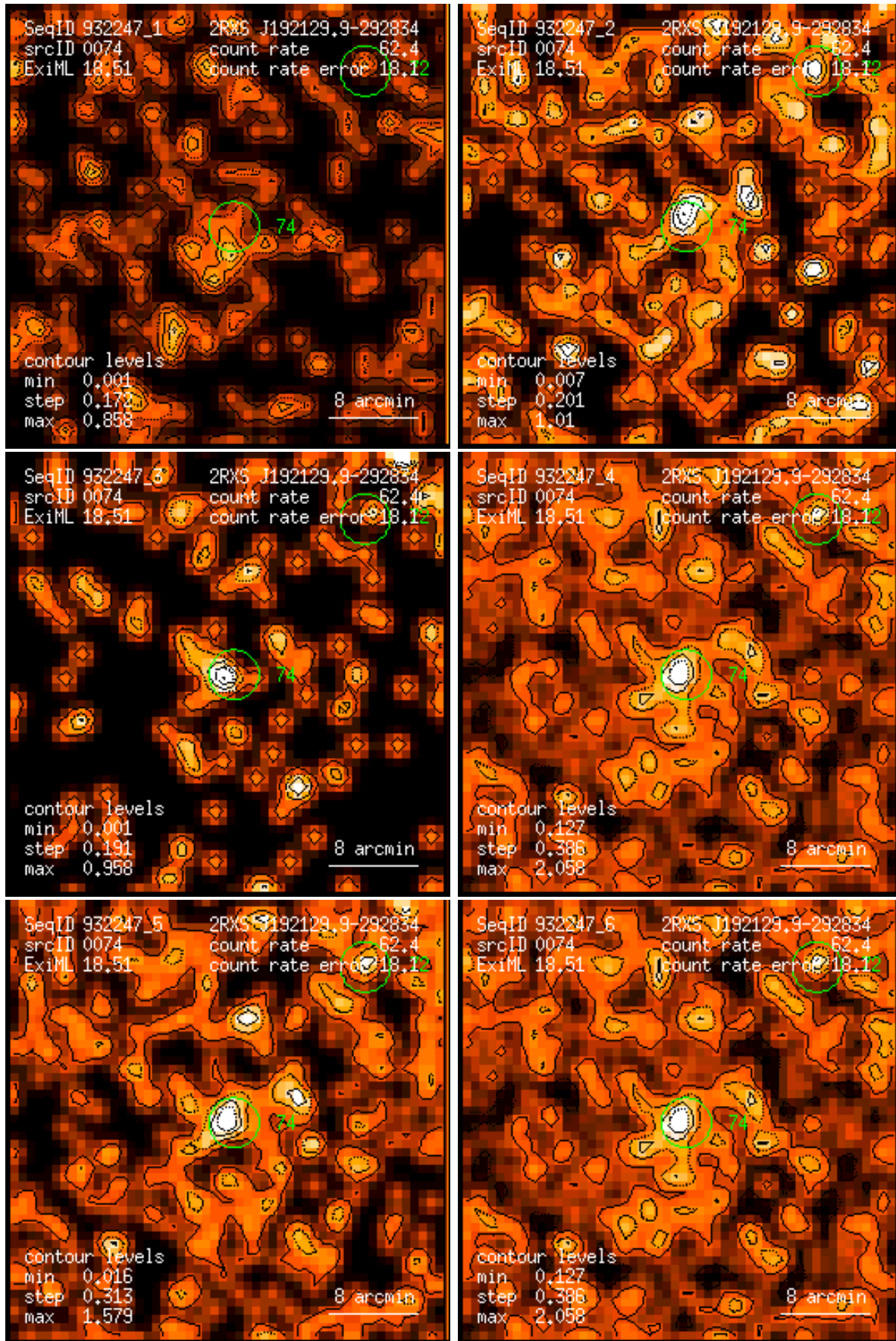
Figure 74: RASS 932247: detection 0074: band rate images, Gaussian filter: (1) PSPC channels 11 – 41, (2) 52 – 90, (3) 91 – 201, (4) 11 – 235, (5) 52 – 201, (6) 11 – 201. Broad band rates in counts/ks. Band rate contour levels in counts/ks/arcmin 2 .
