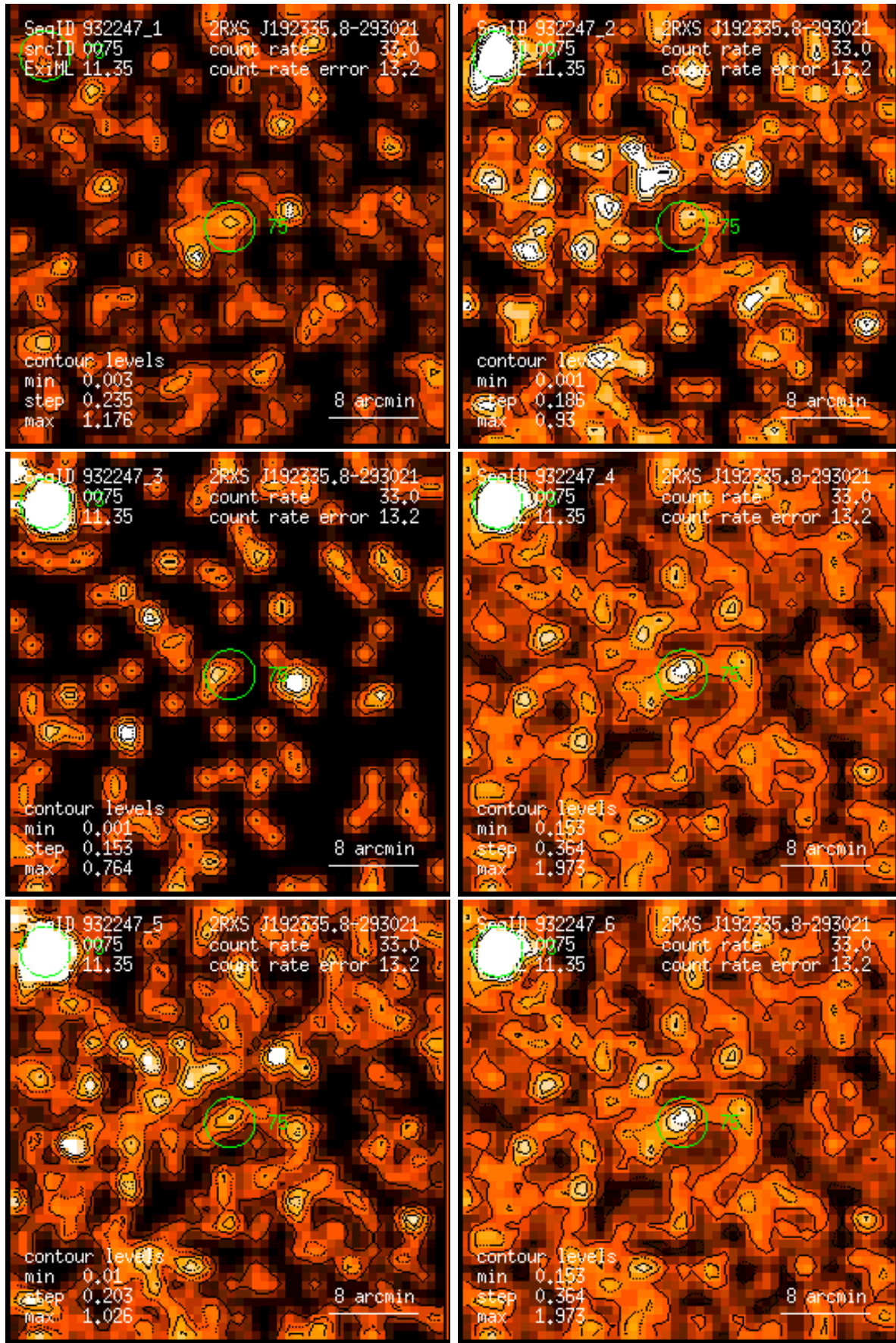
Figure 75: RASS 932247: detection 0075: band rate images, Gaussian filter: (1) PSPC channels 11 – 41, (2) 52 – 90, (3) 91 – 201, (4) 11 – 235, (5) 52 – 201, (6) 11 – 201. Broad band rates in counts/ks. Band rate contour levels in counts/ks/arcmin 2 .
