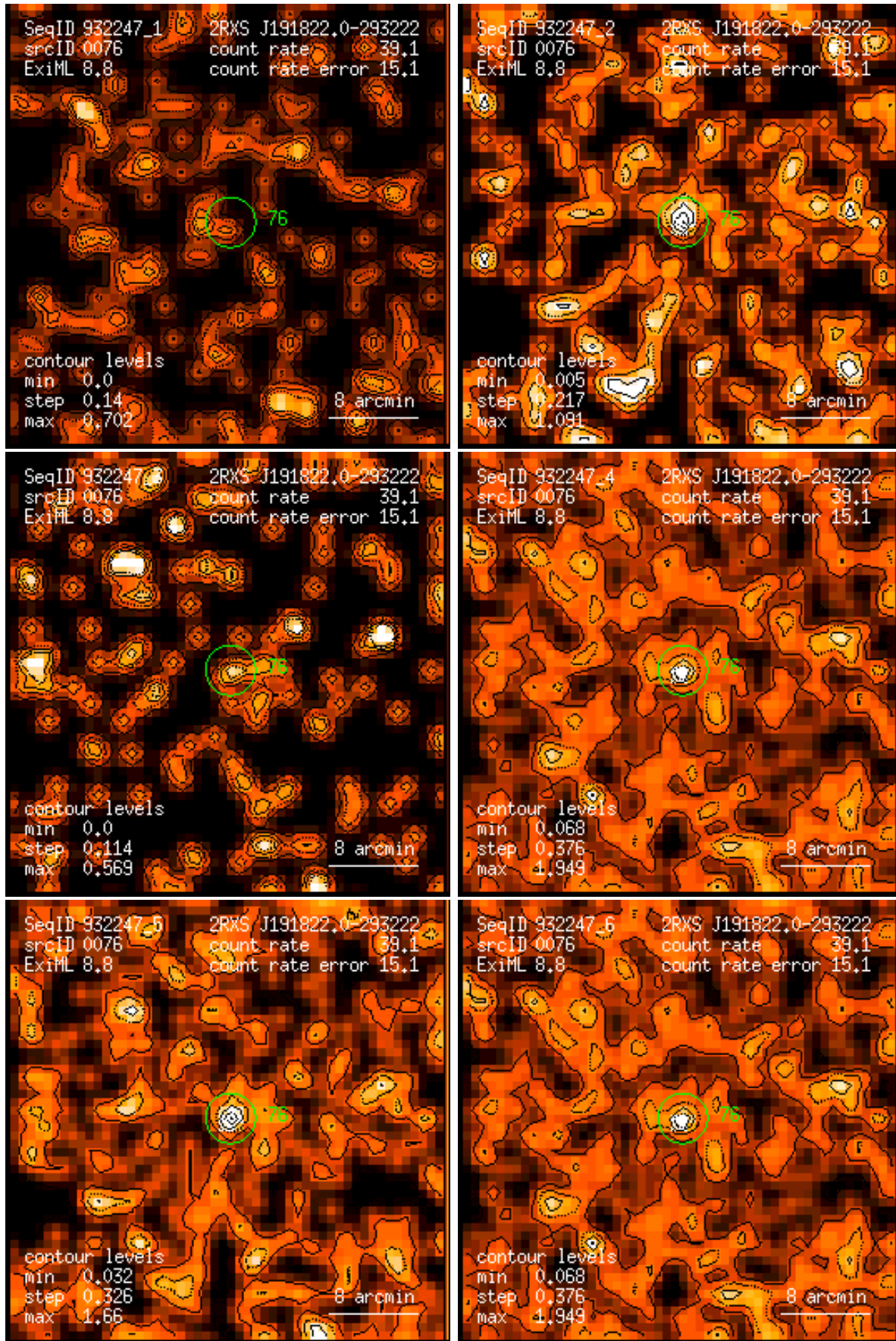
Figure 76: RASS 932247: detection 0076: band rate images, Gaussian filter: (1) PSPC channels 11 – 41, (2) 52 – 90, (3) 91 – 201, (4) 11 – 235, (5) 52 – 201, (6) 11 – 201. Broad band rates in counts/ks. Band rate contour levels in counts/ks/arcmin 2 .
