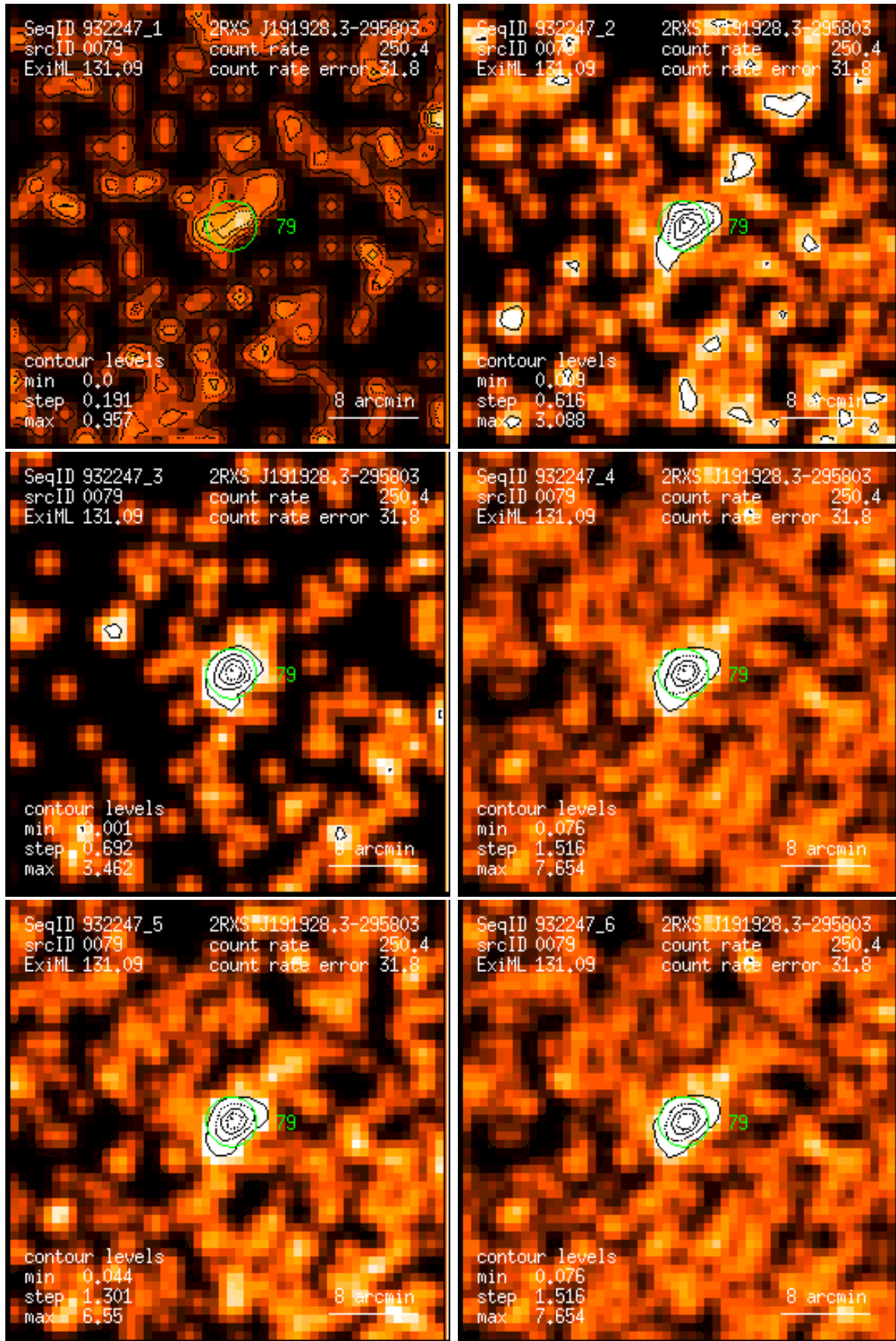
Figure 79: RASS 932247: detection 0079: band rate images, Gaussian filter: (1) PSPC channels 11 – 41, (2) 52 – 90, (3) 91 – 201, (4) 11 – 235, (5) 52 – 201, (6) 11 – 201. Broad band rates in counts/ks. Band rate contour levels in counts/ks/arcmin 2 .
