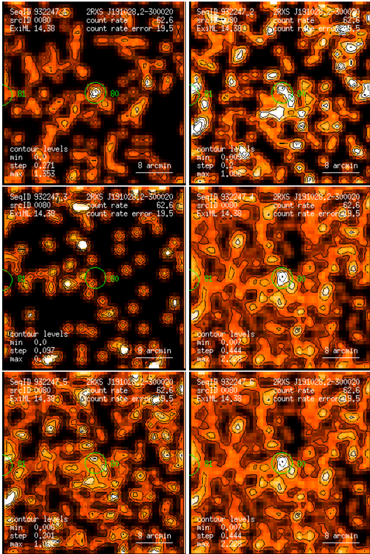
Figure 80: RASS 932247: detection 0080: band rate images, Gaussian filter: (1) PSPC channels 11 – 41, (2) 52 – 90, (3) 91 – 201, (4) 11 – 235, (5) 52 – 201, (6) 11 – 201. Broad band rates in counts/ks. Band rate contour levels in counts/ks/arcmin 2 .
