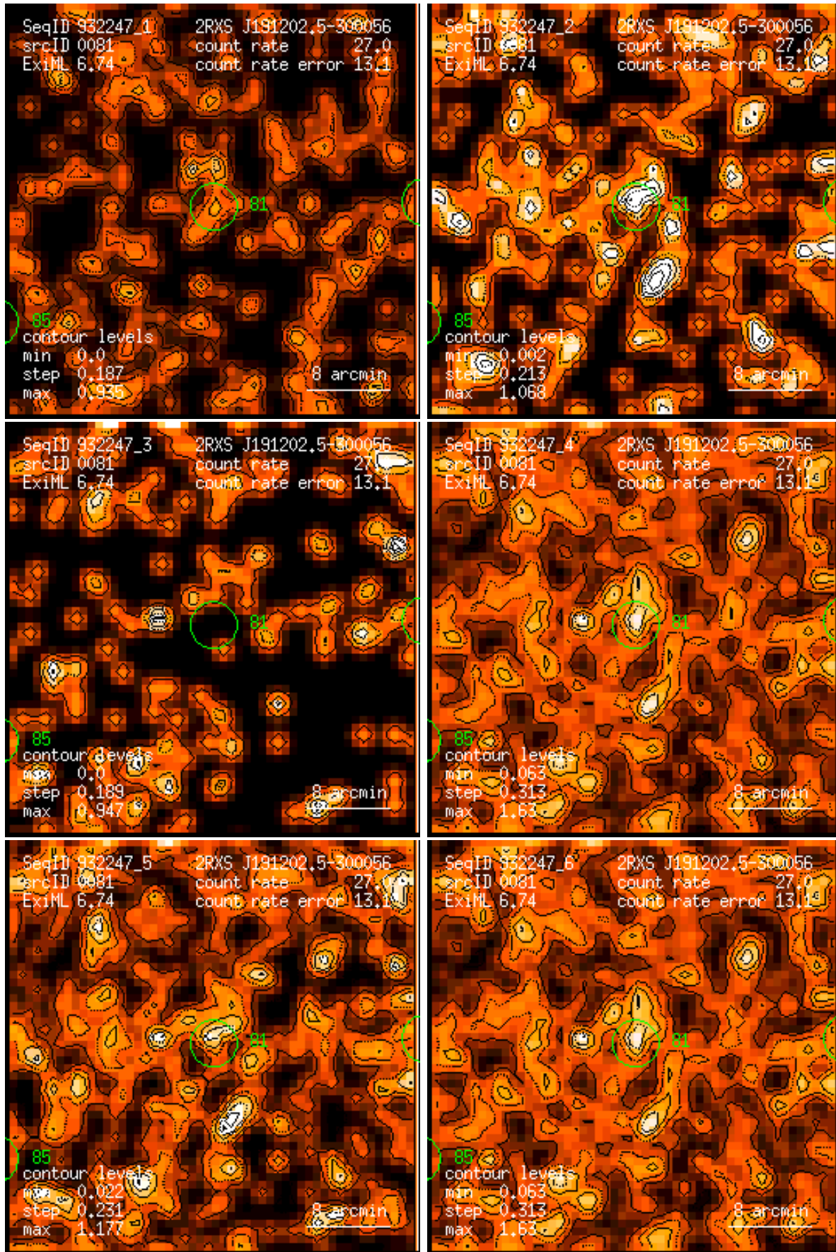
Figure 81: RASS 932247: detection 0081: band rate images, Gaussian filter: (1) PSPC channels 11 – 41, (2) 52 – 90, (3) 91 – 201, (4) 11 – 235, (5) 52 – 201, (6) 11 – 201. Broad band rates in counts/ks. Band rate contour levels in counts/ks/arcmin 2 .
