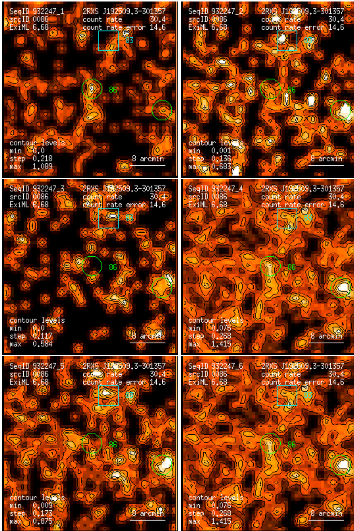
Figure 86: RASS 932247: detection 0086: band rate images, Gaussian filter: (1) PSPC channels 11 – 41, (2) 52 – 90, (3) 91 – 201, (4) 11 – 235, (5) 52 – 201, (6) 11 – 201. Broad band rates in counts/ks. Band rate contour levels in counts/ks/arcmin 2 .
