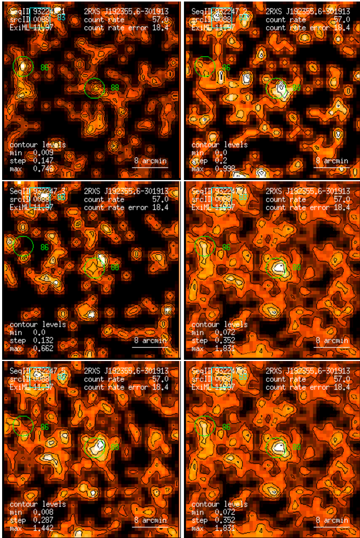
Figure 88: RASS 932247: detection 0088: band rate images, Gaussian filter: (1) PSPC channels 11 – 41, (2) 52 – 90, (3) 91 – 201, (4) 11 – 235, (5) 52 – 201, (6) 11 – 201. Broad band rates in counts/ks. Band rate contour levels in counts/ks/arcmin 2 .
