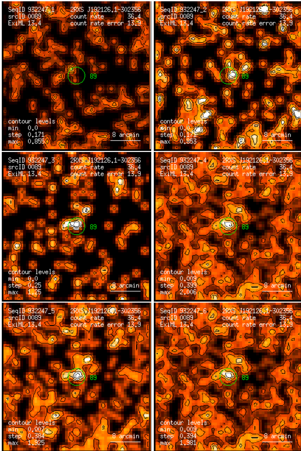
Figure 89: RASS 932247: detection 0089: band rate images, Gaussian filter: (1) PSPC channels 11 – 41, (2) 52 – 90, (3) 91 – 201, (4) 11 – 235, (5) 52 – 201, (6) 11 – 201. Broad band rates in counts/ks. Band rate contour levels in counts/ks/arcmin 2 .
