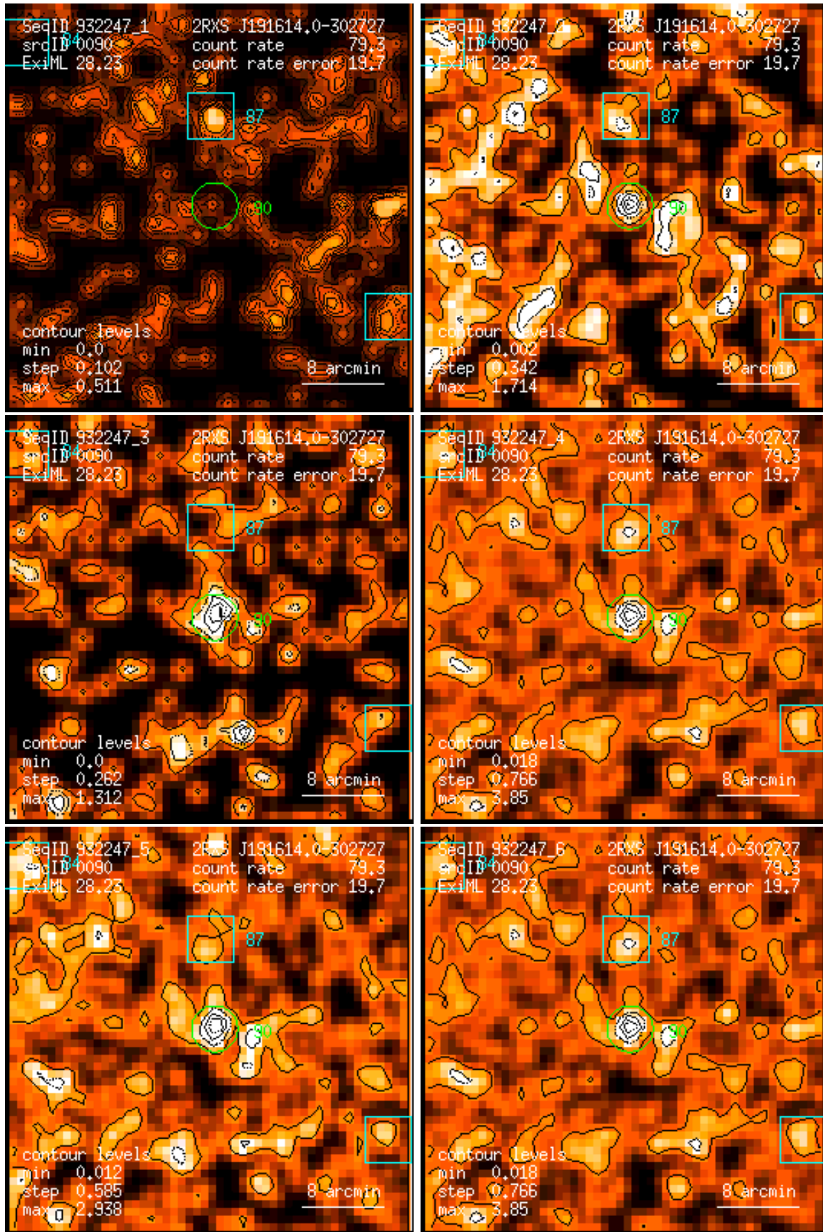
Figure 90: RASS 932247: detection 0090: band rate images, Gaussian filter: (1) PSPC channels 11 – 41, (2) 52 – 90, (3) 91 – 201, (4) 11 – 235, (5) 52 – 201, (6) 11 – 201. Broad band rates in counts/ks. Band rate contour levels in counts/ks/arcmin 2 .
