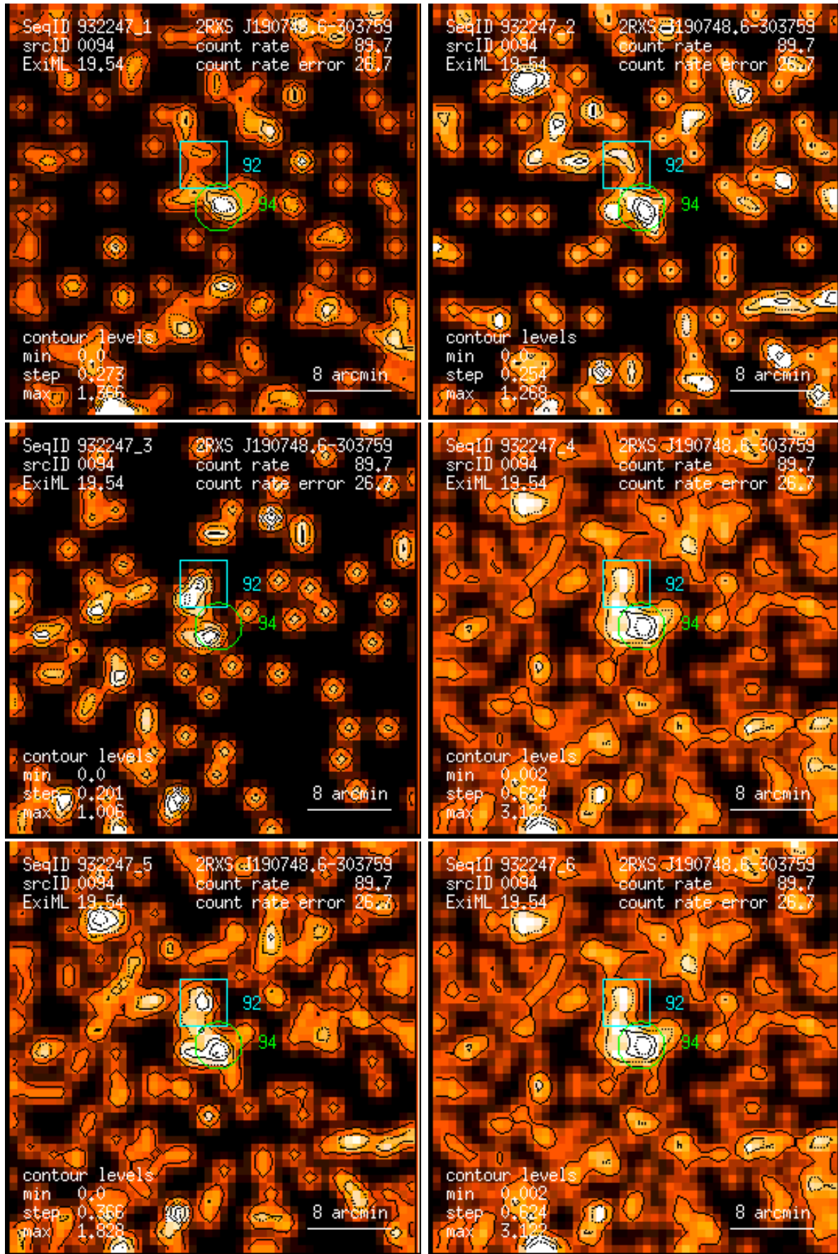
Figure 94: RASS 932247: detection 0094: band rate images, Gaussian filter: (1) PSPC channels 11 – 41, (2) 52 – 90, (3) 91 – 201, (4) 11 – 235, (5) 52 – 201, (6) 11 – 201. Broad band rates in counts/ks. Band rate contour levels in counts/ks/arcmin 2 .
