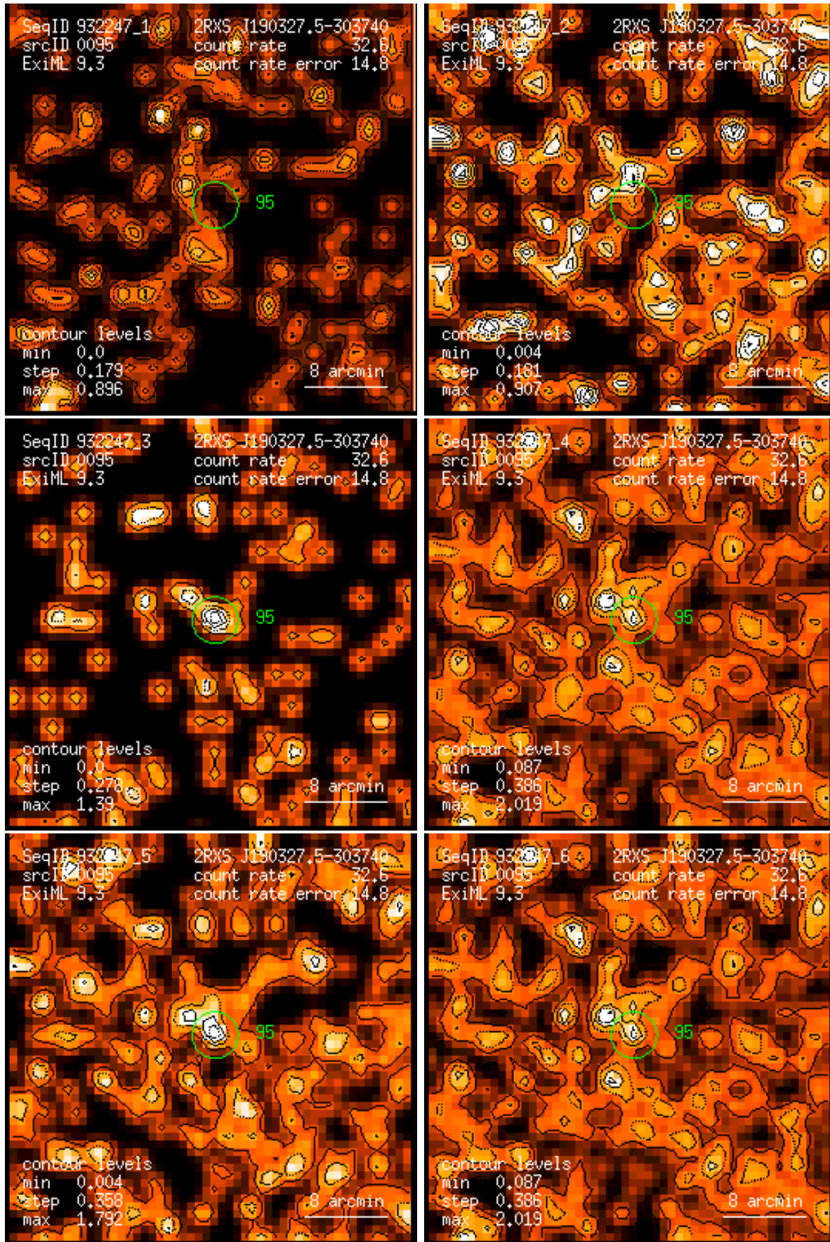
Figure 95: RASS 932247: detection 0095: band rate images, Gaussian filter: (1) PSPC channels 11 – 41, (2) 52 – 90, (3) 91 – 201, (4) 11 – 235, (5) 52 – 201, (6) 11 – 201. Broad band rates in counts/ks. Band rate contour levels in counts/ks/arcmin 2 .
