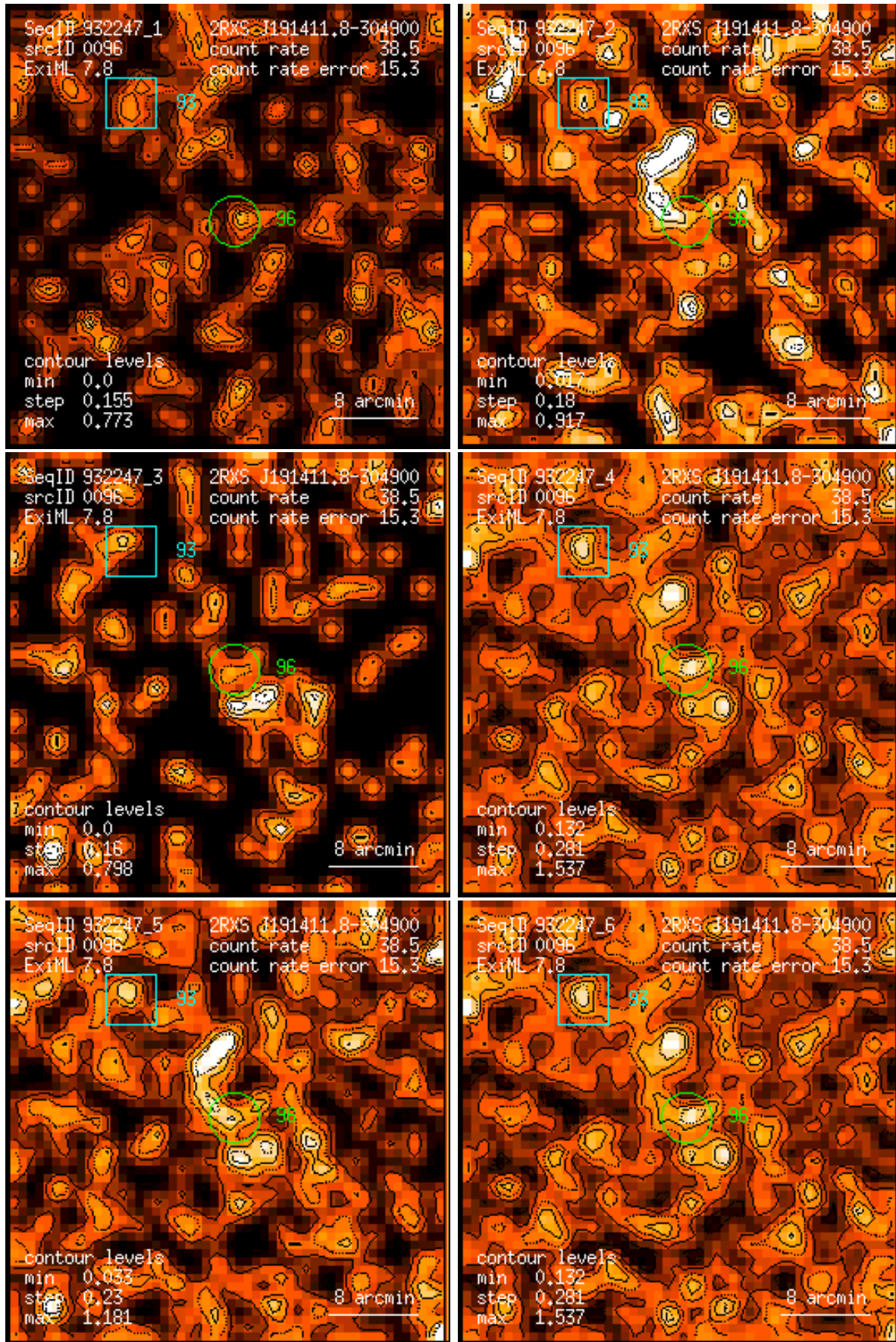
Figure 96: RASS 932247: detection 0096: band rate images, Gaussian filter: (1) PSPC channels 11 – 41, (2) 52 – 90, (3) 91 – 201, (4) 11 – 235, (5) 52 – 201, (6) 11 – 201. Broad band rates in counts/ks. Band rate contour levels in counts/ks/arcmin 2 .
