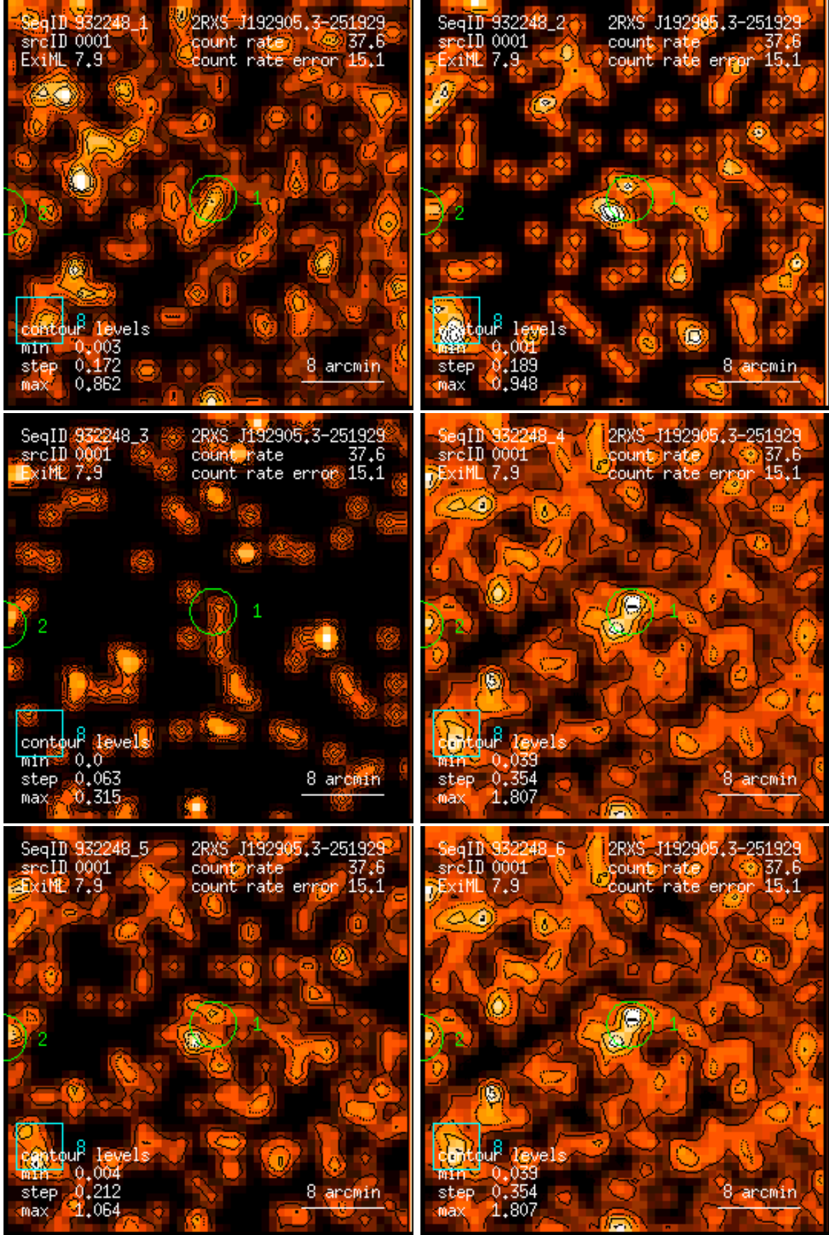
Figure 1: RASS 932248: detection 0001: band rate images, Gaussian filter: (1) PSPC channels 11 – 41, (2) 52 – 90, (3) 91 – 201, (4) 11 – 235, (5) 52 – 201, (6) 11 – 201. Broad band rates in counts/ks. Band rate contour levels in counts/ks/arcmin 2 .
