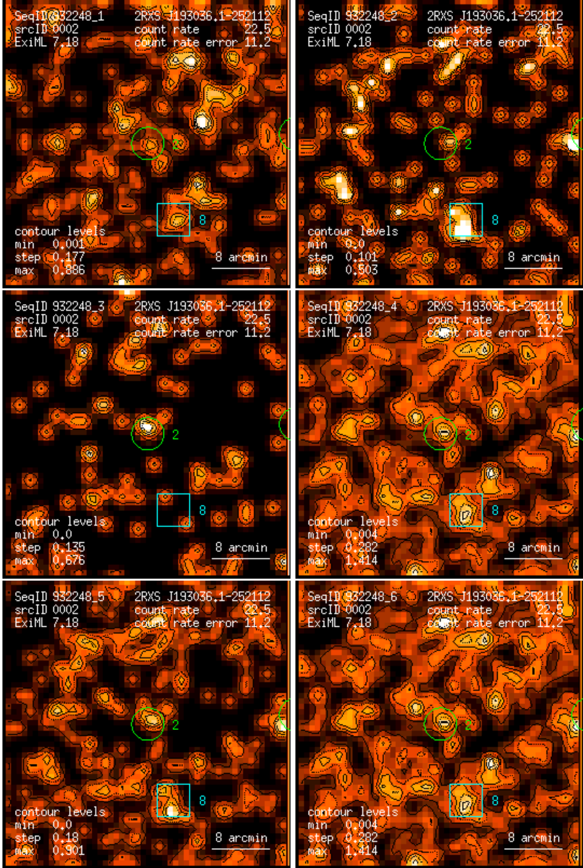
Figure 2: RASS 932248: detection 0002: band rate images, Gaussian filter: (1) PSPC channels 11 – 41, (2) 52 – 90, (3) 91 – 201, (4) 11 – 235, (5) 52 – 201, (6) 11 – 201. Broad band rates in counts/ks. Band rate contour levels in counts/ks/arcmin 2 .
