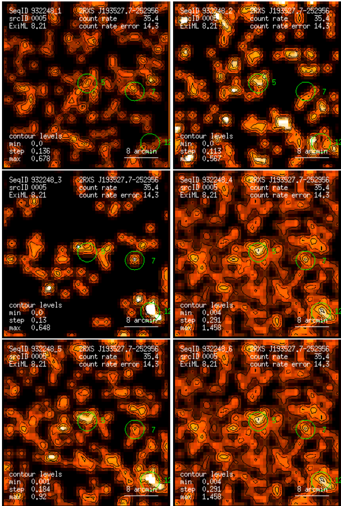
Figure 5: RASS 932248: detection 0005: band rate images, Gaussian filter: (1) PSPC channels 11 – 41, (2) 52 – 90, (3) 91 – 201, (4) 11 – 235, (5) 52 – 201, (6) 11 – 201. Broad band rates in counts/ks. Band rate contour levels in counts/ks/arcmin 2 .
