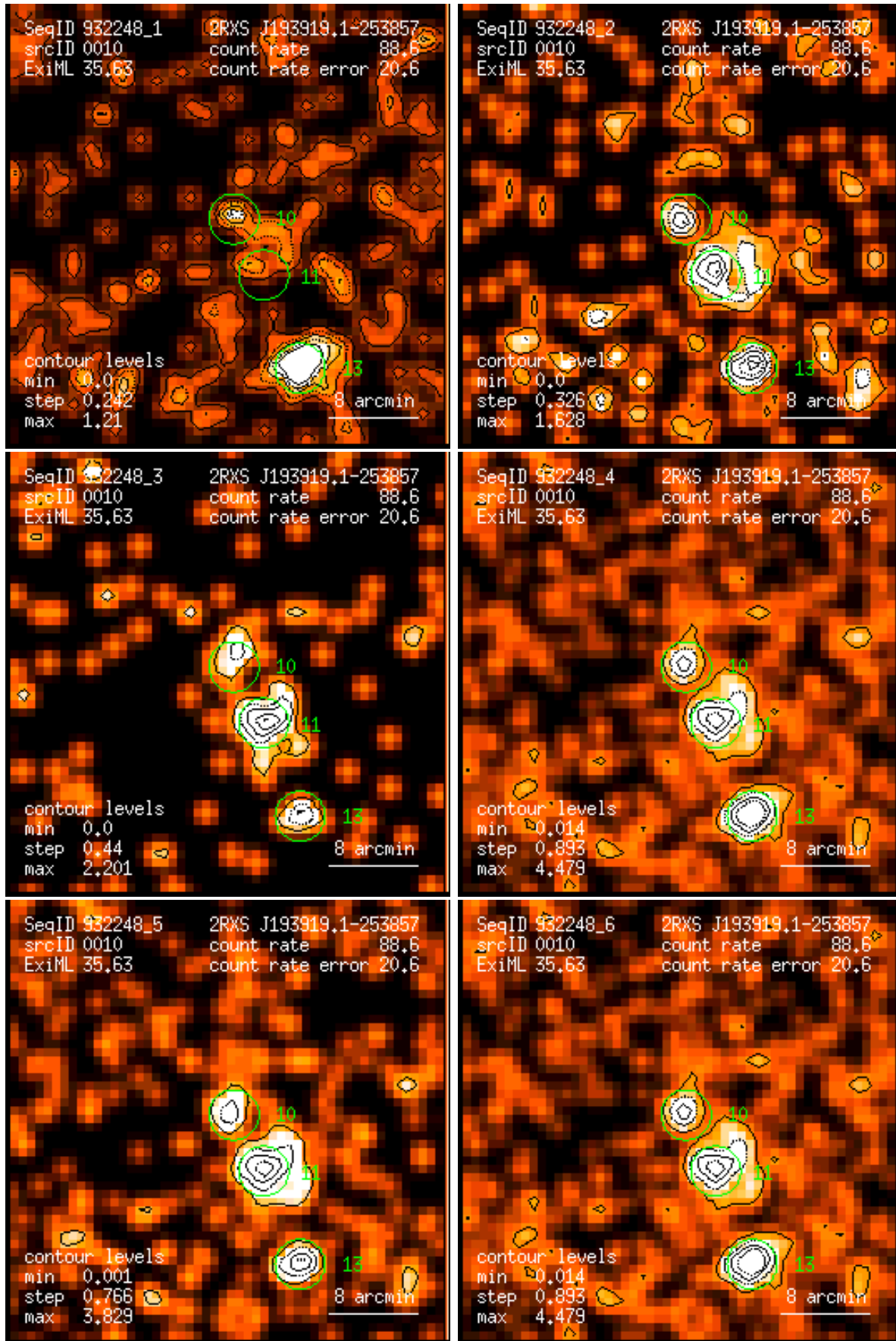
Figure 10: RASS 932248: detection 0010: band rate images, Gaussian filter: (1) PSPC channels 11 – 41, (2) 52 – 90, (3) 91 – 201, (4) 11 – 235, (5) 52 – 201, (6) 11 – 201. Broad band rates in counts/ks. Band rate contour levels in counts/ks/arcmin 2 .
