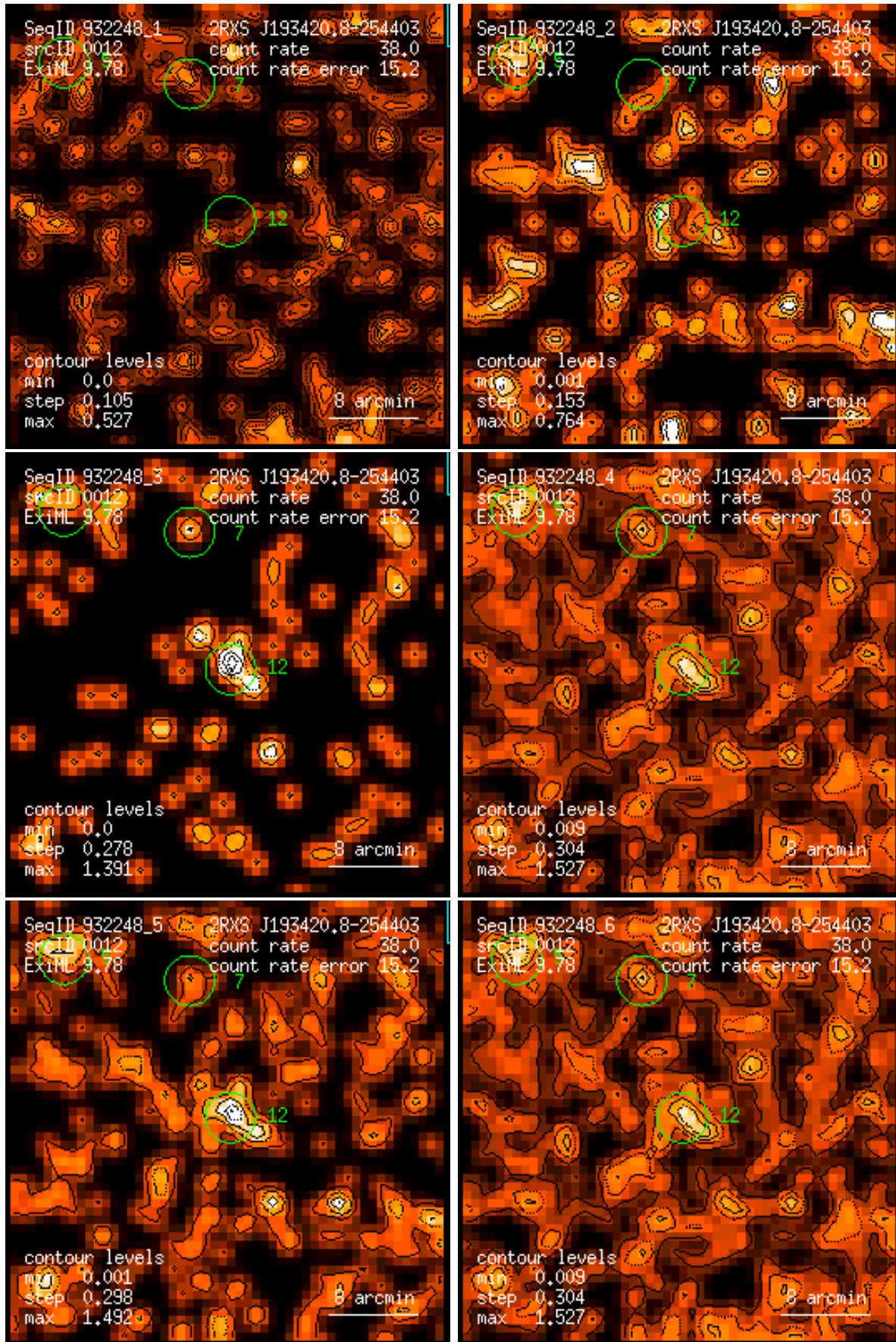
Figure 12: RASS 932248: detection 0012: band rate images, Gaussian filter: (1) PSPC channels 11 – 41, (2) 52 – 90, (3) 91 – 201, (4) 11 – 235, (5) 52 – 201, (6) 11 – 201. Broad band rates in counts/ks. Band rate contour levels in counts/ks/arcmin 2 .
