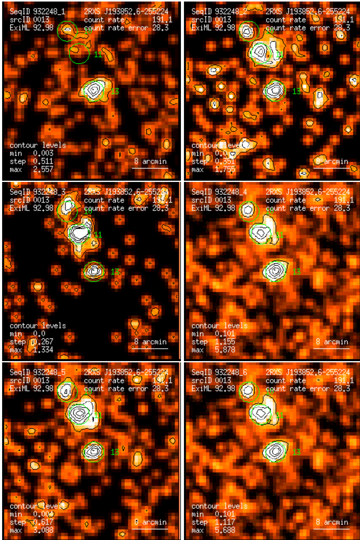
Figure 13: RASS 932248: detection 0013: band rate images, Gaussian filter: (1) PSPC channels 11 – 41, (2) 52 – 90, (3) 91 – 201, (4) 11 – 235, (5) 52 – 201, (6) 11 – 201. Broad band rates in counts/ks. Band rate contour levels in counts/ks/arcmin 2 .
