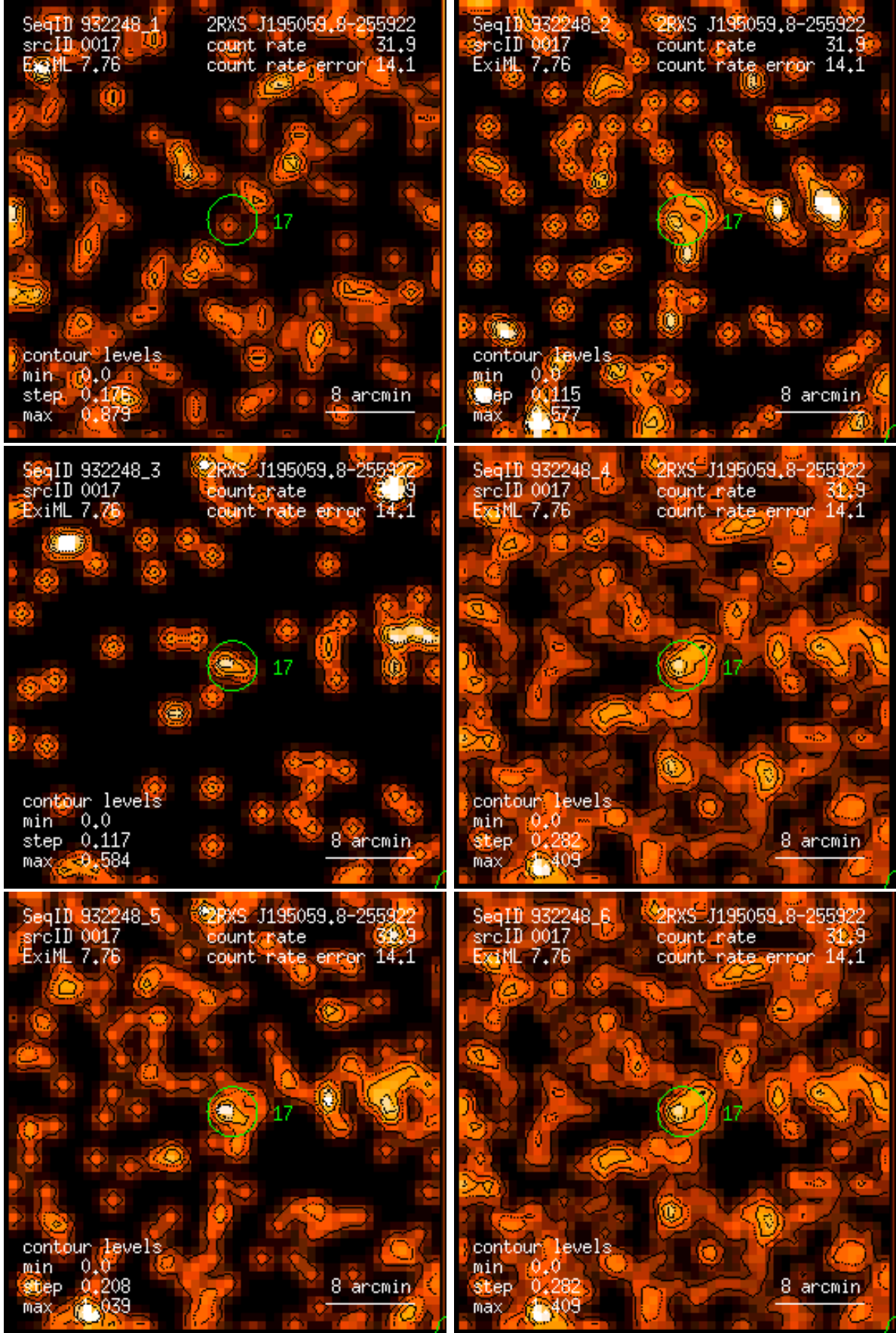
Figure 17: RASS 932248: detection 0017: band rate images, Gaussian filter: (1) PSPC channels 11 – 41, (2) 52 – 90, (3) 91 – 201, (4) 11 – 235, (5) 52 – 201, (6) 11 – 201. Broad band rates in counts/ks. Band rate contour levels in counts/ks/arcmin 2 .
