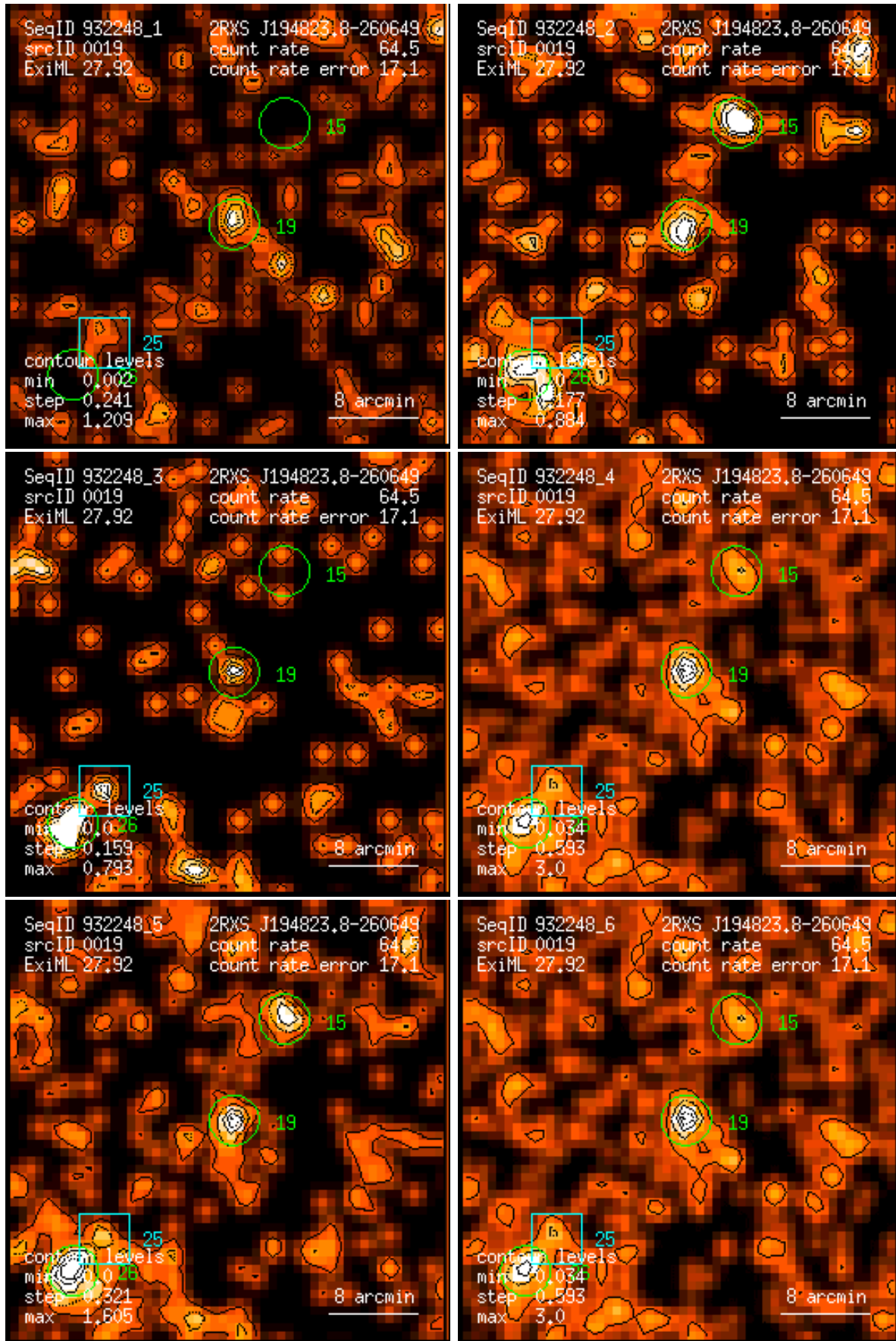
Figure 19: RASS 932248: detection 0019: band rate images, Gaussian filter: (1) PSPC channels 11 – 41, (2) 52 – 90, (3) 91 – 201, (4) 11 – 235, (5) 52 – 201, (6) 11 – 201. Broad band rates in counts/ks. Band rate contour levels in counts/ks/arcmin 2 .
