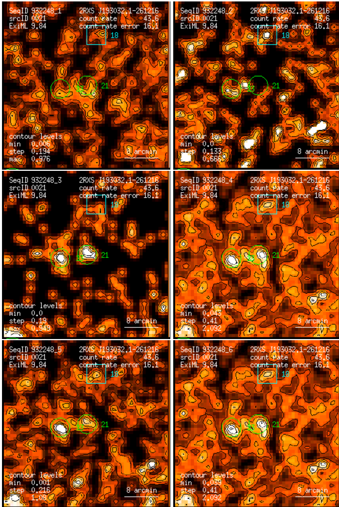
Figure 21: RASS 932248: detection 0021: band rate images, Gaussian filter: (1) PSPC channels 11 – 41, (2) 52 – 90, (3) 91 – 201, (4) 11 – 235, (5) 52 – 201, (6) 11 – 201. Broad band rates in counts/ks. Band rate contour levels in counts/ks/arcmin 2 .
