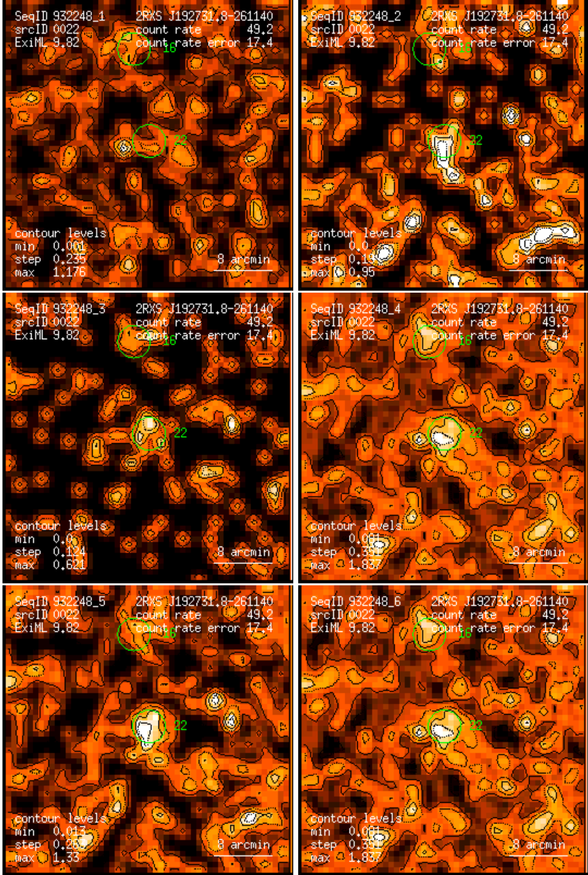
Figure 22: RASS 932248: detection 0022: band rate images, Gaussian filter: (1) PSPC channels 11 – 41, (2) 52 – 90, (3) 91 – 201, (4) 11 – 235, (5) 52 – 201, (6) 11 – 201. Broad band rates in counts/ks. Band rate contour levels in counts/ks/arcmin 2 .
