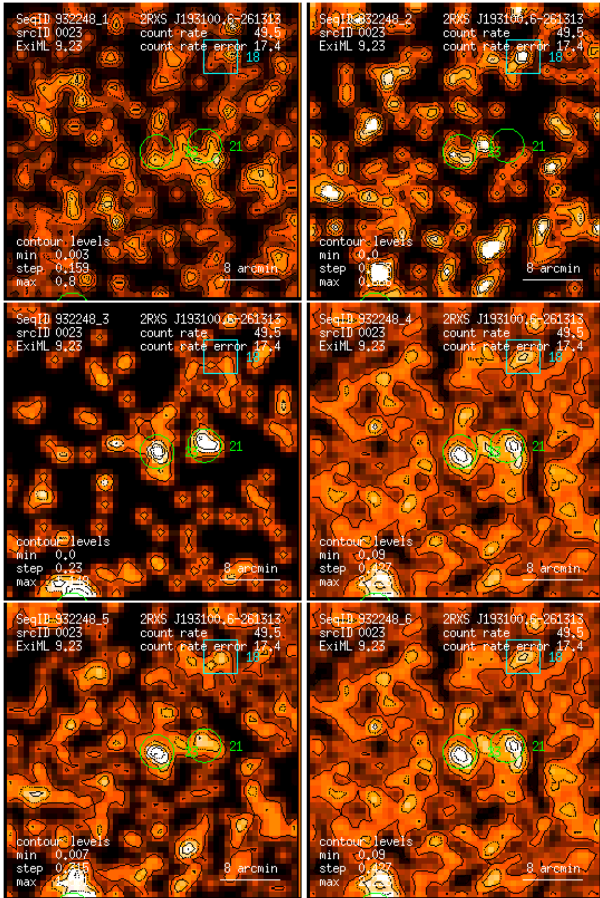
Figure 23: RASS 932248: detection 0023: band rate images, Gaussian filter: (1) PSPC channels 11 – 41, (2) 52 – 90, (3) 91 – 201, (4) 11 – 235, (5) 52 – 201, (6) 11 – 201. Broad band rates in counts/ks. Band rate contour levels in counts/ks/arcmin 2 .
