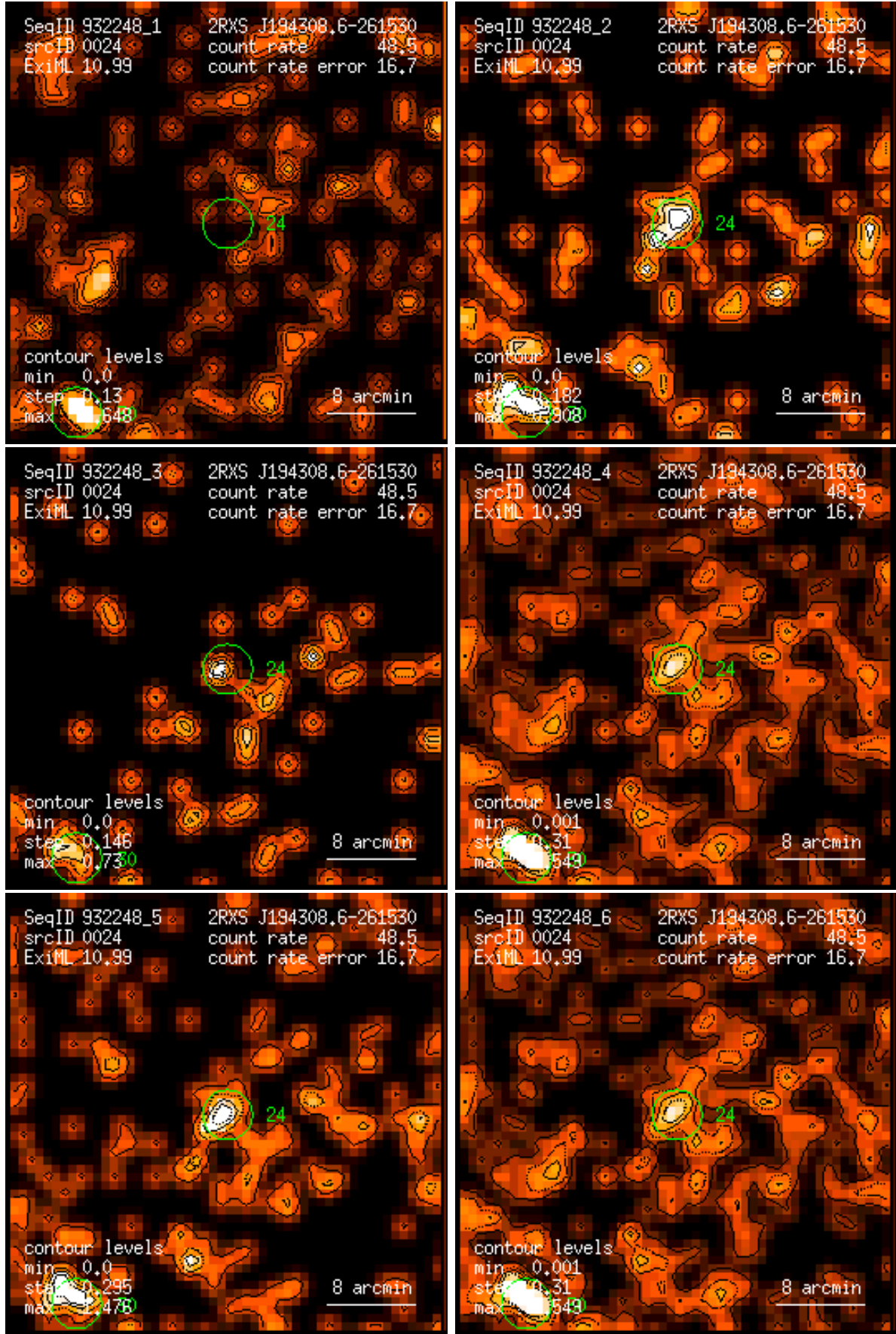
Figure 24: RASS 932248: detection 0024: band rate images, Gaussian filter: (1) PSPC channels 11 – 41, (2) 52 – 90, (3) 91 – 201, (4) 11 – 235, (5) 52 – 201, (6) 11 – 201. Broad band rates in counts/ks. Band rate contour levels in counts/ks/arcmin 2 .
