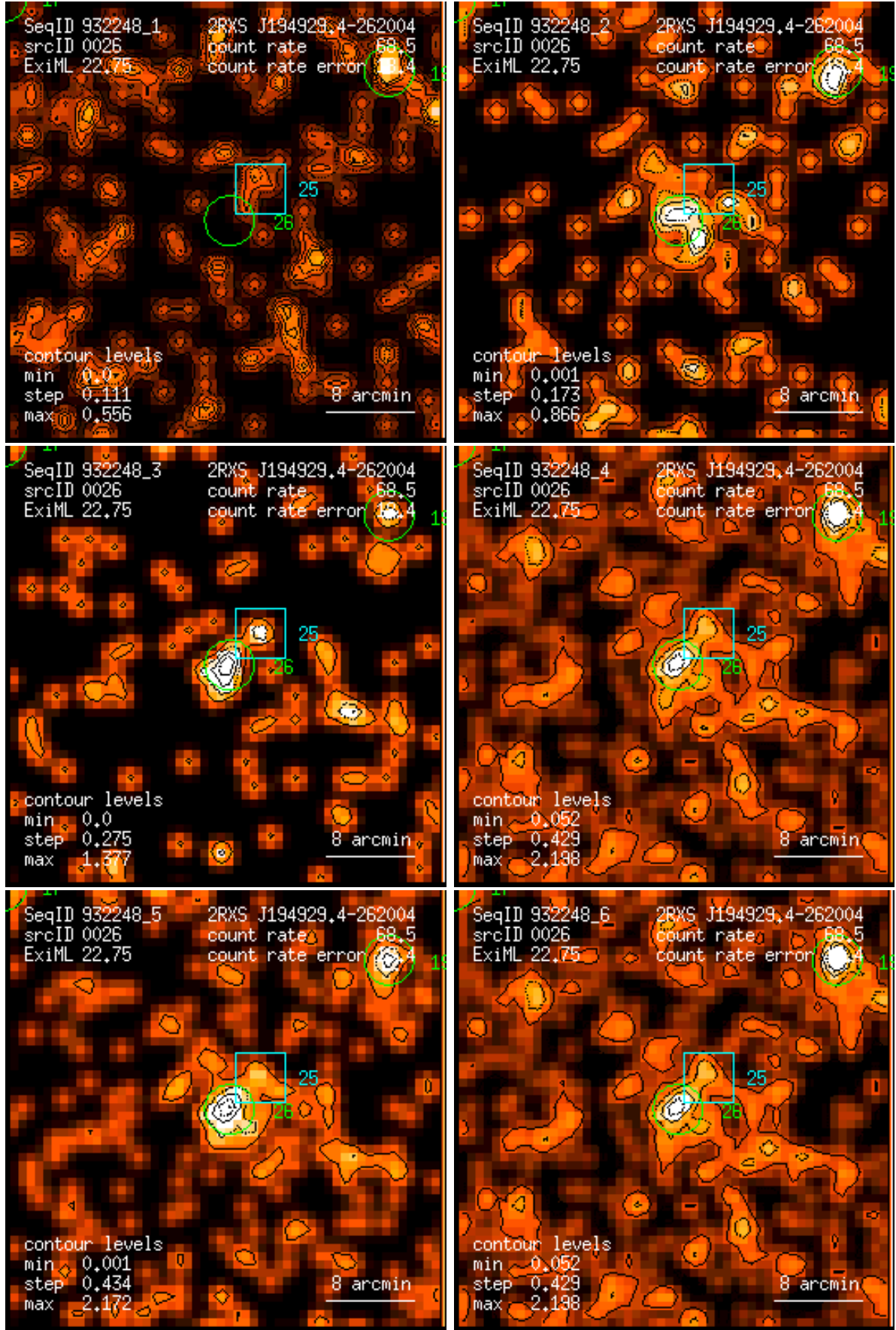
Figure 26: RASS 932248: detection 0026: band rate images, Gaussian filter: (1) PSPC channels 11 – 41, (2) 52 – 90, (3) 91 – 201, (4) 11 – 235, (5) 52 – 201, (6) 11 – 201. Broad band rates in counts/ks. Band rate contour levels in counts/ks/arcmin 2 .
