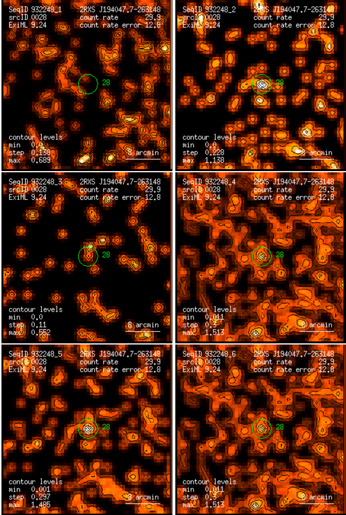
Figure 28: RASS 932248: detection 0028: band rate images, Gaussian filter: (1) PSPC channels 11 – 41, (2) 52 – 90, (3) 91 – 201, (4) 11 – 235, (5) 52 – 201, (6) 11 – 201. Broad band rates in counts/ks. Band rate contour levels in counts/ks/arcmin 2 .
