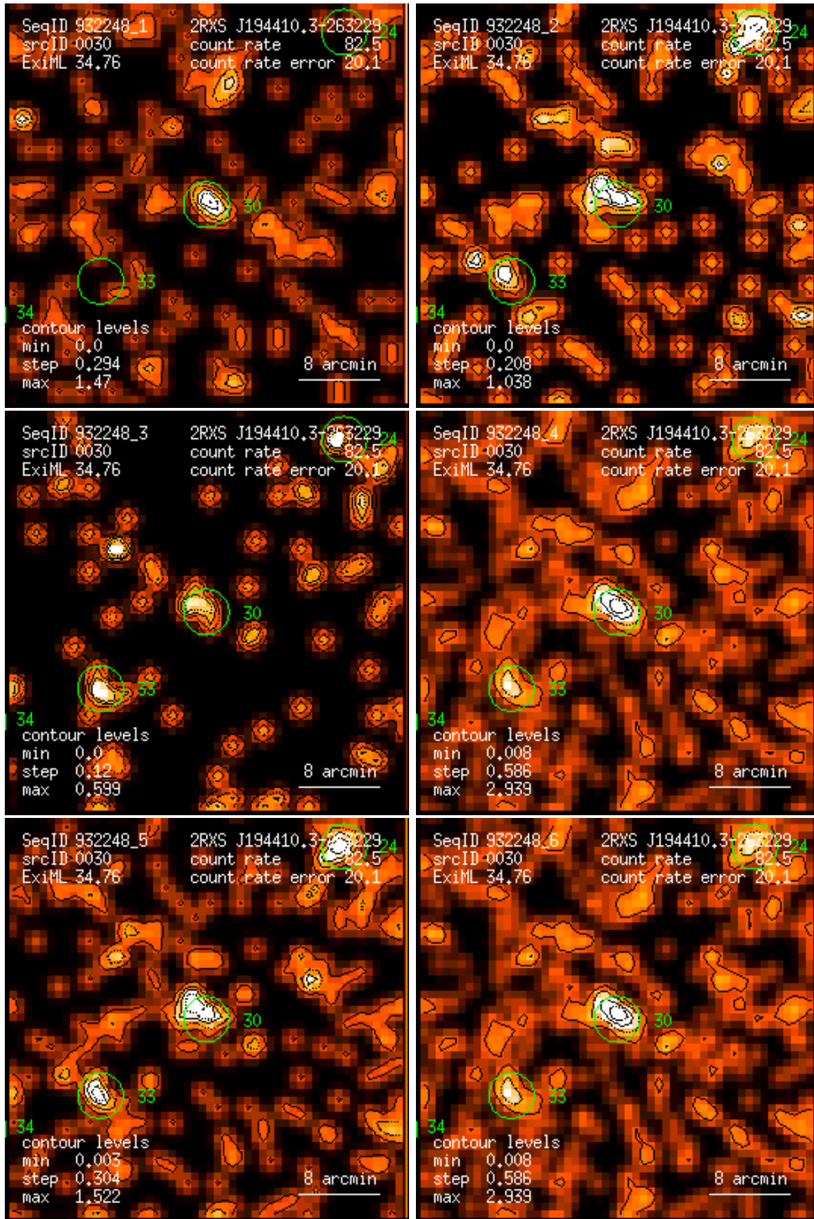
Figure 30: RASS 932248: detection 0030: band rate images, Gaussian filter: (1) PSPC channels 11 – 41, (2) 52 – 90, (3) 91 – 201, (4) 11 – 235, (5) 52 – 201, (6) 11 – 201. Broad band rates in counts/ks. Band rate contour levels in counts/ks/arcmin 2 .
