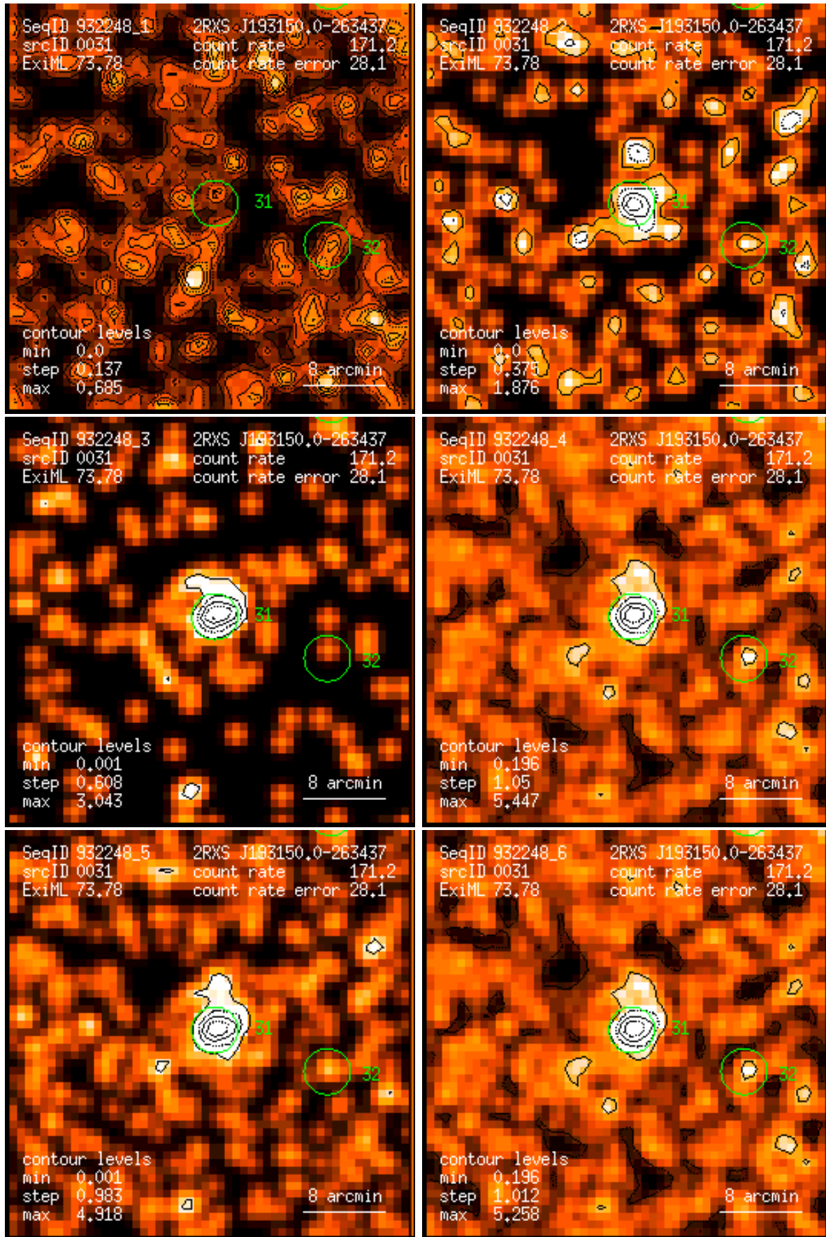
Figure 31: RASS 932248: detection 0031: band rate images, Gaussian filter: (1) PSPC channels 11 – 41, (2) 52 – 90, (3) 91 – 201, (4) 11 – 235, (5) 52 – 201, (6) 11 – 201. Broad band rates in counts/ks. Band rate contour levels in counts/ks/arcmin 2 .
