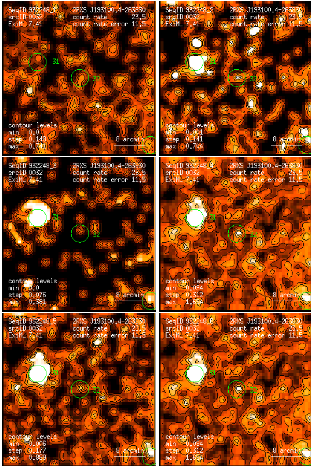
Figure 32: RASS 932248: detection 0032: band rate images, Gaussian filter: (1) PSPC channels 11 – 41, (2) 52 – 90, (3) 91 – 201, (4) 11 – 235, (5) 52 – 201, (6) 11 – 201. Broad band rates in counts/ks. Band rate contour levels in counts/ks/arcmin 2 .
