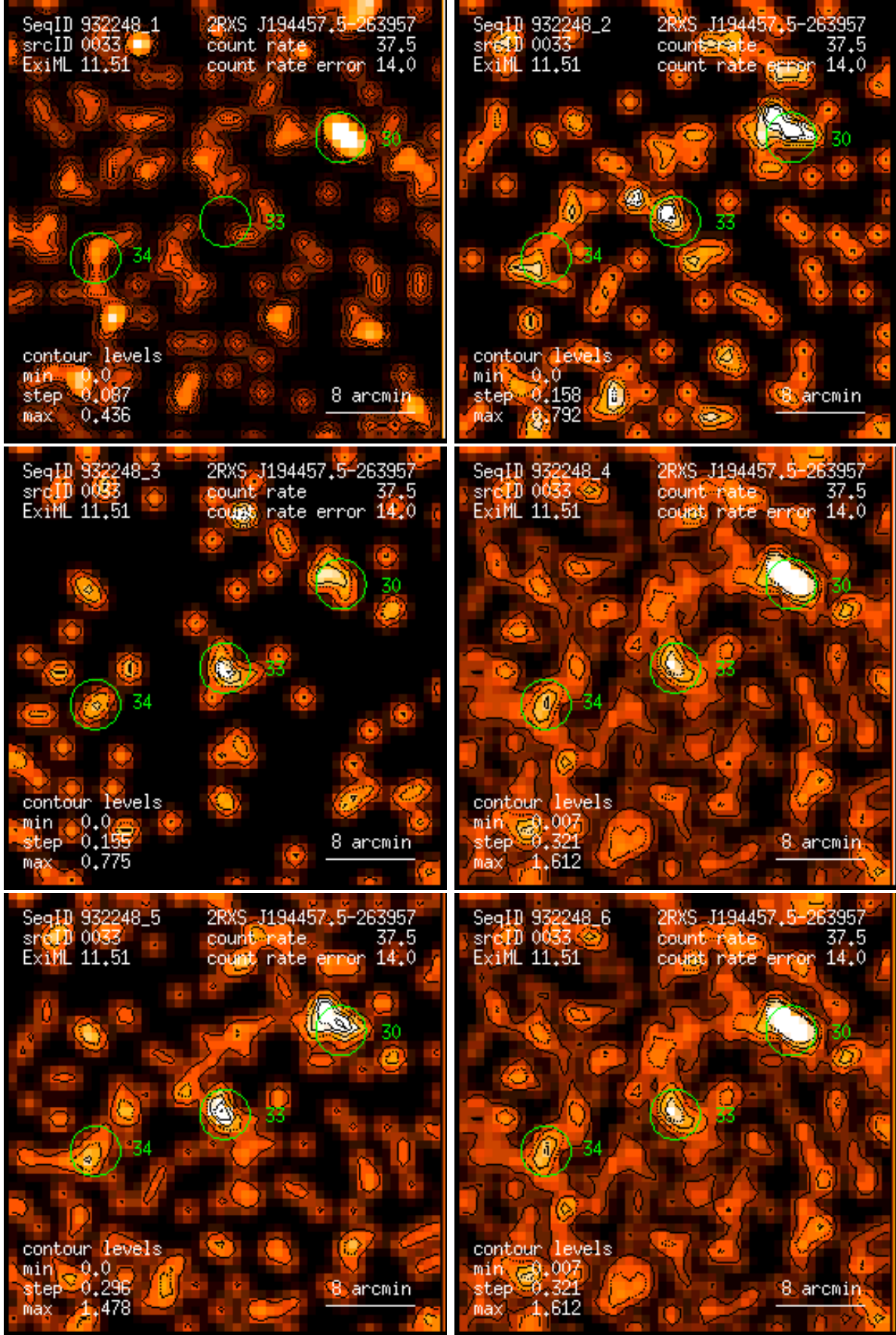
Figure 33: RASS 932248: detection 0033: band rate images, Gaussian filter: (1) PSPC channels 11 – 41, (2) 52 – 90, (3) 91 – 201, (4) 11 – 235, (5) 52 – 201, (6) 11 – 201. Broad band rates in counts/ks. Band rate contour levels in counts/ks/arcmin 2 .
