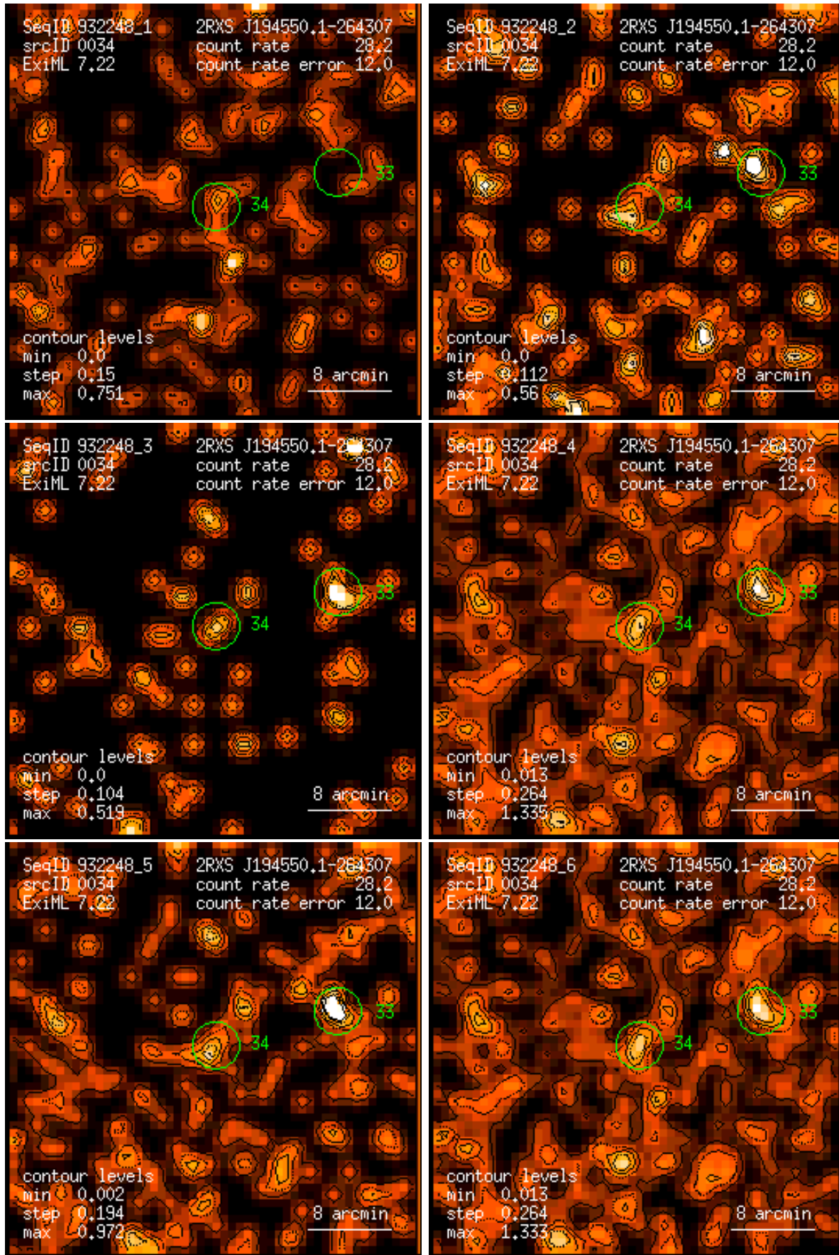
Figure 34: RASS 932248: detection 0034: band rate images, Gaussian filter: (1) PSPC channels 11 – 41, (2) 52 – 90, (3) 91 – 201, (4) 11 – 235, (5) 52 – 201, (6) 11 – 201. Broad band rates in counts/ks. Band rate contour levels in counts/ks/arcmin 2 .
