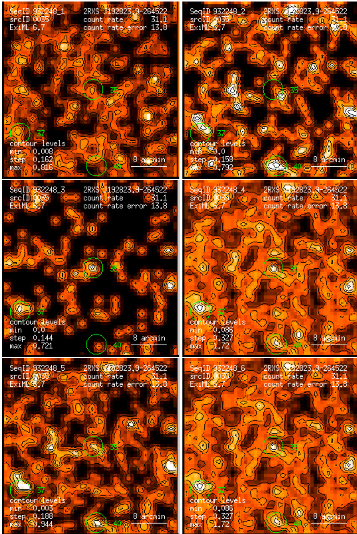
Figure 35: RASS 932248: detection 0035: band rate images, Gaussian filter: (1) PSPC channels 11 – 41, (2) 52 – 90, (3) 91 – 201, (4) 11 – 235, (5) 52 – 201, (6) 11 – 201. Broad band rates in counts/ks. Band rate contour levels in counts/ks/arcmin 2 .
