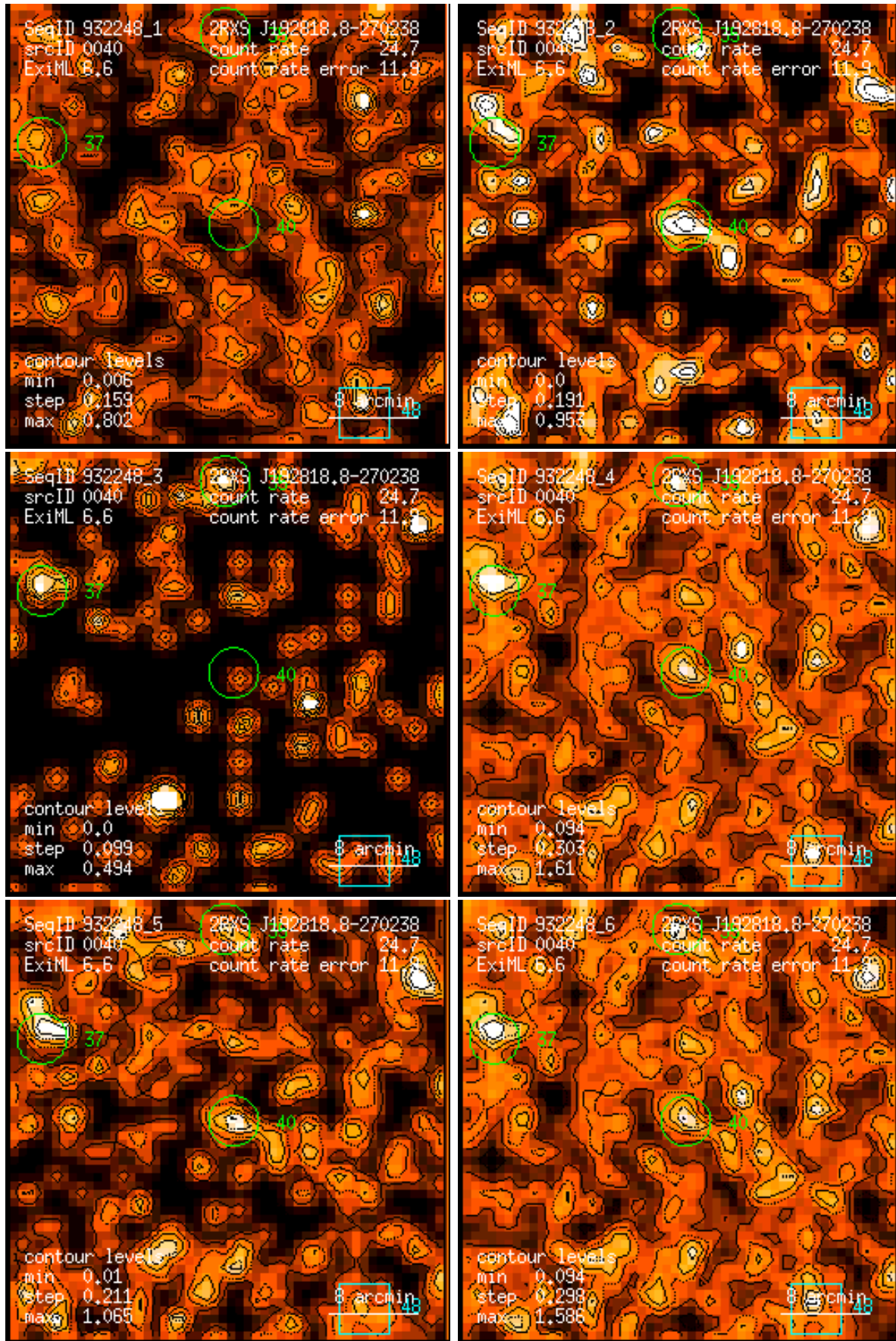
Figure 40: RASS 932248: detection 0040: band rate images, Gaussian filter: (1) PSPC channels 11 – 41, (2) 52 – 90, (3) 91 – 201, (4) 11 – 235, (5) 52 – 201, (6) 11 – 201. Broad band rates in counts/ks. Band rate contour levels in counts/ks/arcmin 2 .
