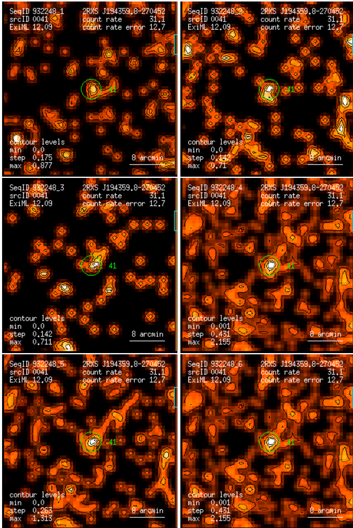
Figure 41: RASS 932248: detection 0041: band rate images, Gaussian filter: (1) PSPC channels 11 – 41, (2) 52 – 90, (3) 91 – 201, (4) 11 – 235, (5) 52 – 201, (6) 11 – 201. Broad band rates in counts/ks. Band rate contour levels in counts/ks/arcmin 2 .
