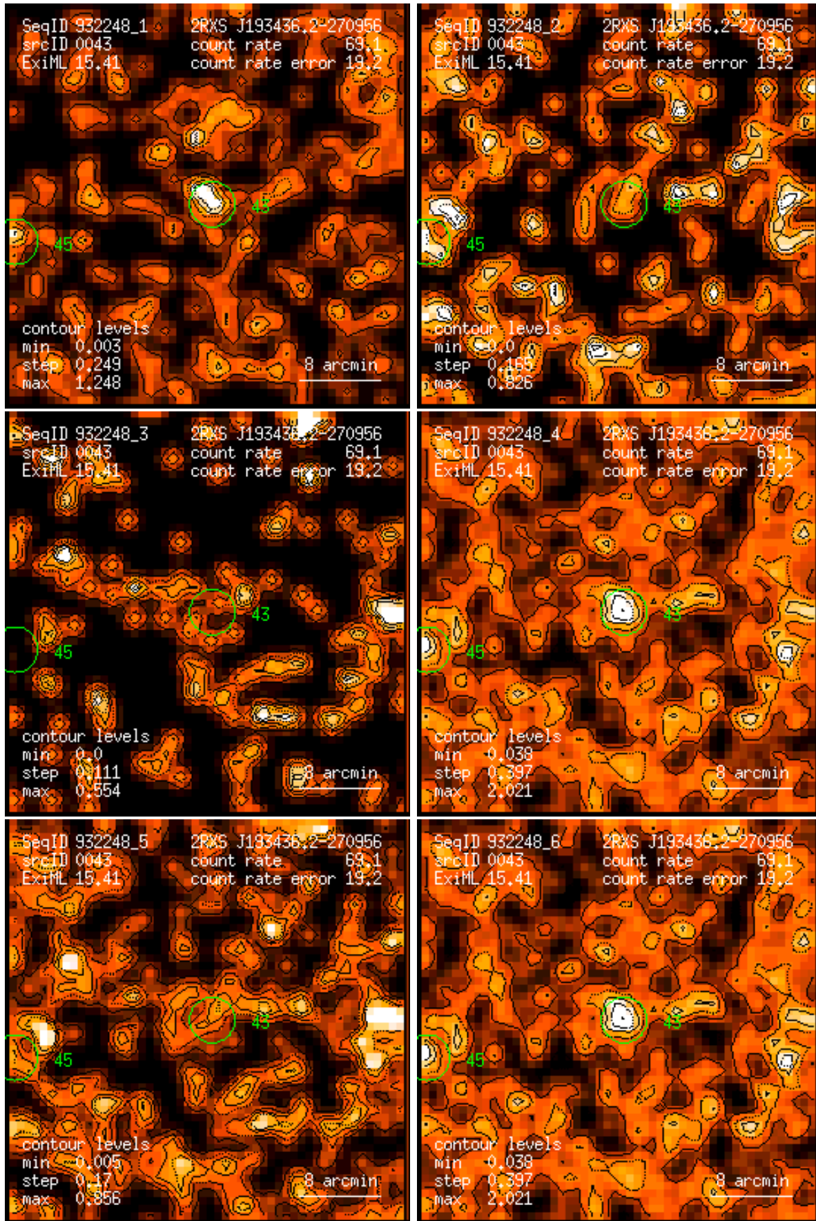
Figure 43: RASS 932248: detection 0043: band rate images, Gaussian filter: (1) PSPC channels 11 – 41, (2) 52 – 90, (3) 91 – 201, (4) 11 – 235, (5) 52 – 201, (6) 11 – 201. Broad band rates in counts/ks. Band rate contour levels in counts/ks/arcmin 2 .
