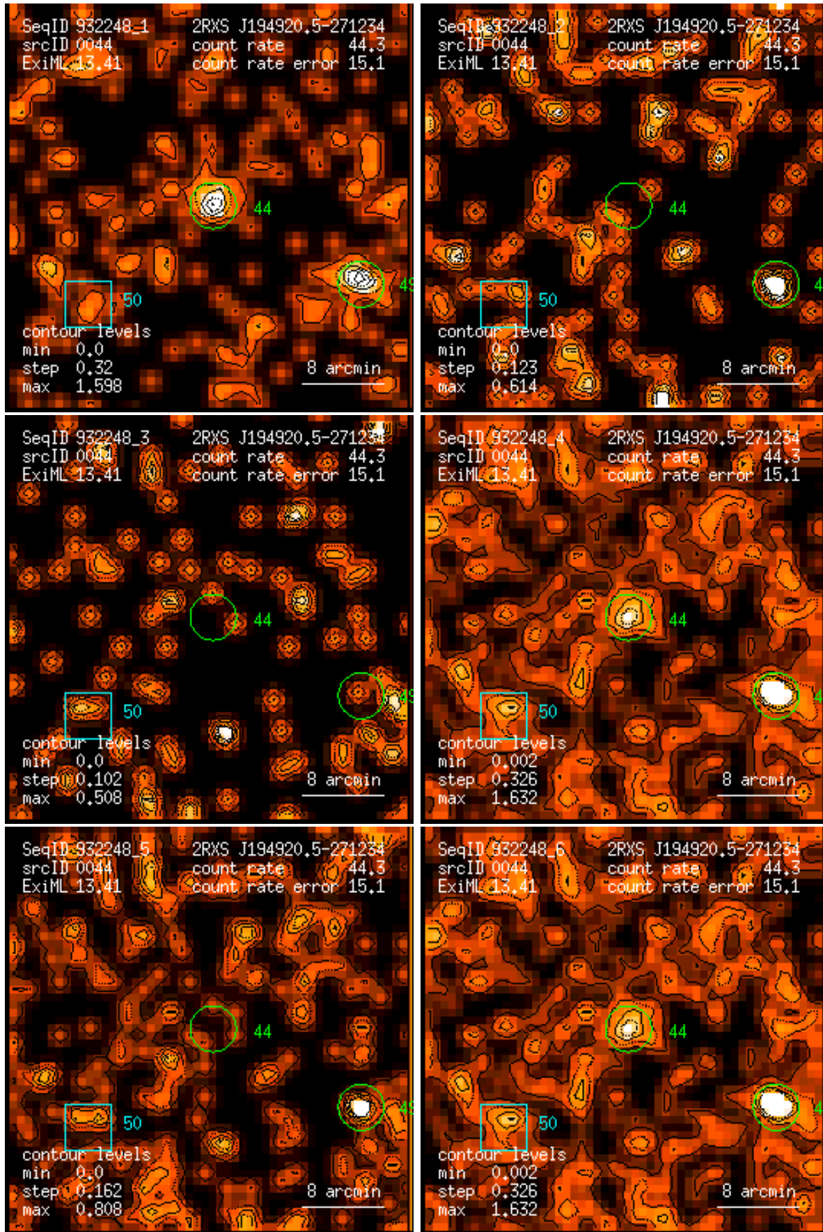
Figure 44: RASS 932248: detection 0044: band rate images, Gaussian filter: (1) PSPC channels 11 – 41, (2) 52 – 90, (3) 91 – 201, (4) 11 – 235, (5) 52 – 201, (6) 11 – 201. Broad band rates in counts/ks. Band rate contour levels in counts/ks/arcmin 2 .
