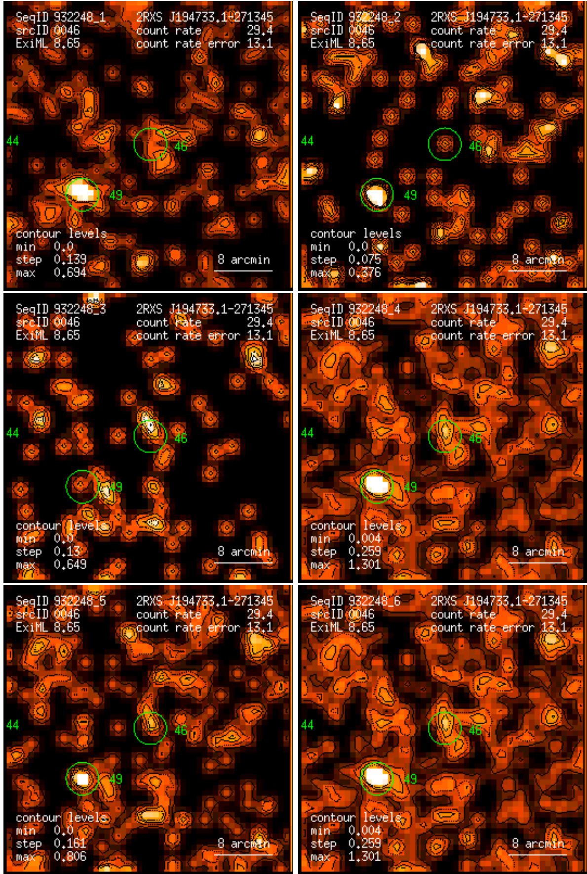
Figure 46: RASS 932248: detection 0046: band rate images, Gaussian filter: (1) PSPC channels 11 – 41, (2) 52 – 90, (3) 91 – 201, (4) 11 – 235, (5) 52 – 201, (6) 11 – 201. Broad band rates in counts/ks. Band rate contour levels in counts/ks/arcmin 2 .
