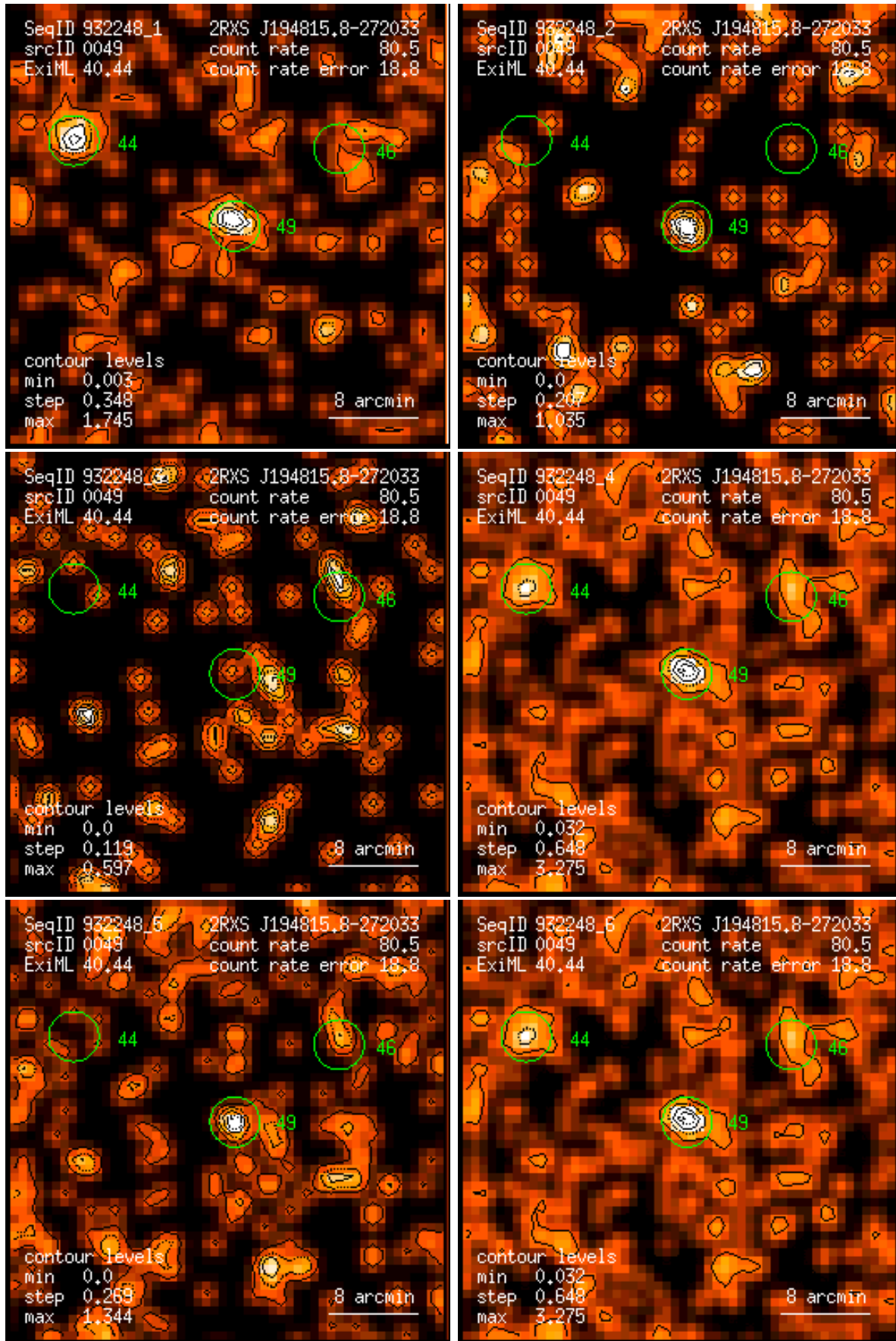
Figure 49: RASS 932248: detection 0049: band rate images, Gaussian filter: (1) PSPC channels 11 – 41, (2) 52 – 90, (3) 91 – 201, (4) 11 – 235, (5) 52 – 201, (6) 11 – 201. Broad band rates in counts/ks. Band rate contour levels in counts/ks/arcmin 2 .
