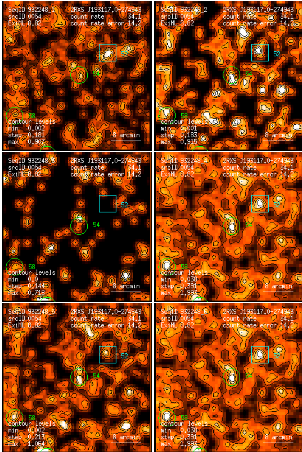
Figure 54: RASS 932248: detection 0054: band rate images, Gaussian filter: (1) PSPC channels 11 – 41, (2) 52 – 90, (3) 91 – 201, (4) 11 – 235, (5) 52 – 201, (6) 11 – 201. Broad band rates in counts/ks. Band rate contour levels in counts/ks/arcmin 2 .
