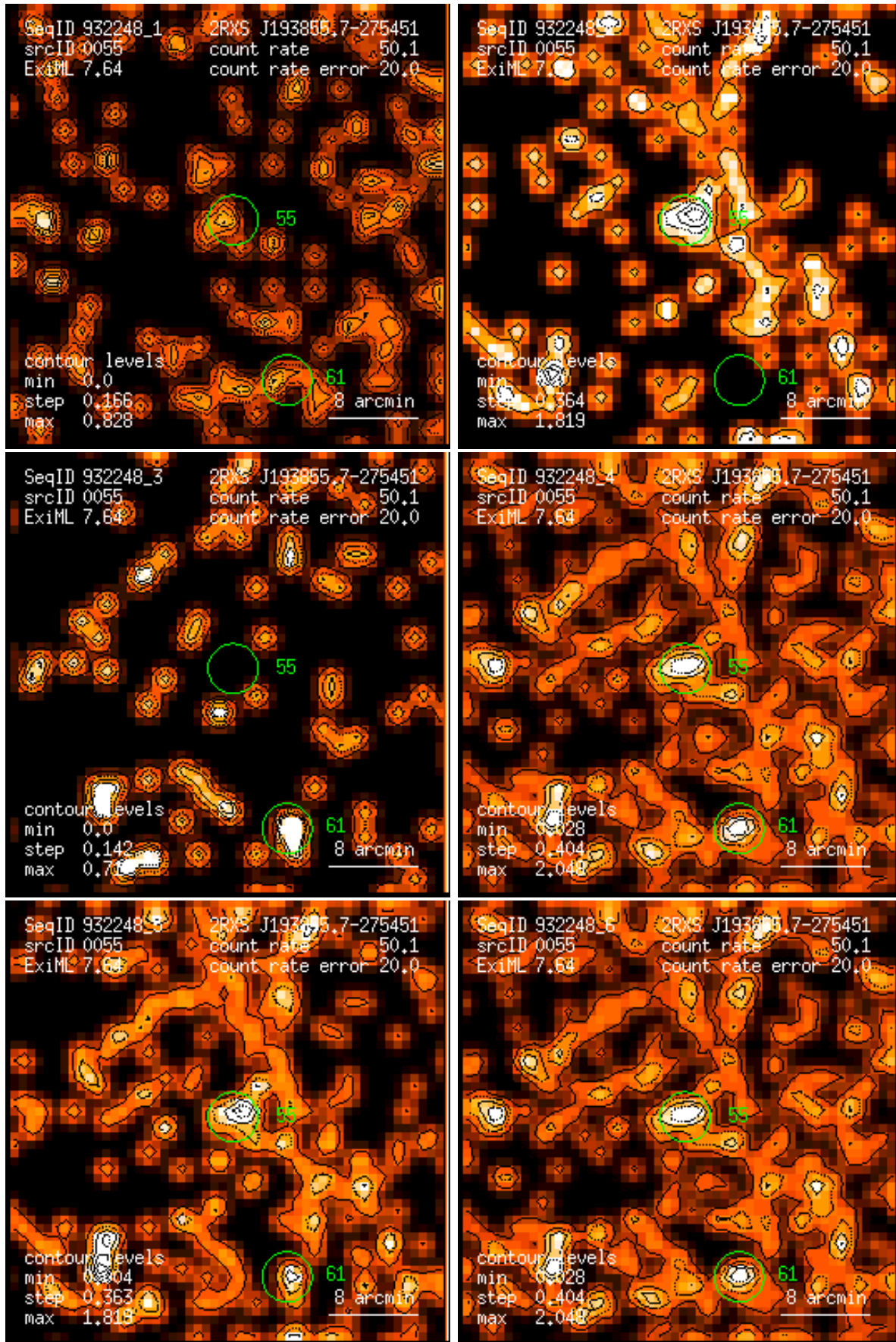
Figure 55: RASS 932248: detection 0055: band rate images, Gaussian filter: (1) PSPC channels 11 – 41, (2) 52 – 90, (3) 91 – 201, (4) 11 – 235, (5) 52 – 201, (6) 11 – 201. Broad band rates in counts/ks. Band rate contour levels in counts/ks/arcmin 2 .
