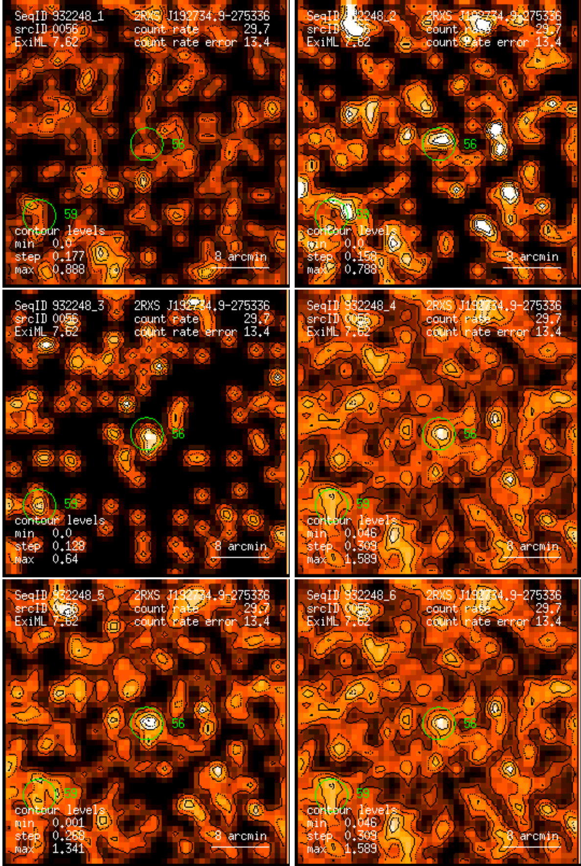
Figure 56: RASS 932248: detection 0056: band rate images, Gaussian filter: (1) PSPC channels 11 – 41, (2) 52 – 90, (3) 91 – 201, (4) 11 – 235, (5) 52 – 201, (6) 11 – 201. Broad band rates in counts/ks. Band rate contour levels in counts/ks/arcmin 2 .
