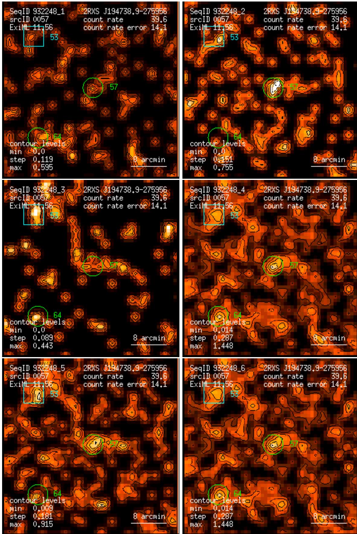
Figure 57: RASS 932248: detection 0057: band rate images, Gaussian filter: (1) PSPC channels 11 – 41, (2) 52 – 90, (3) 91 – 201, (4) 11 – 235, (5) 52 – 201, (6) 11 – 201. Broad band rates in counts/ks. Band rate contour levels in counts/ks/arcmin 2 .
