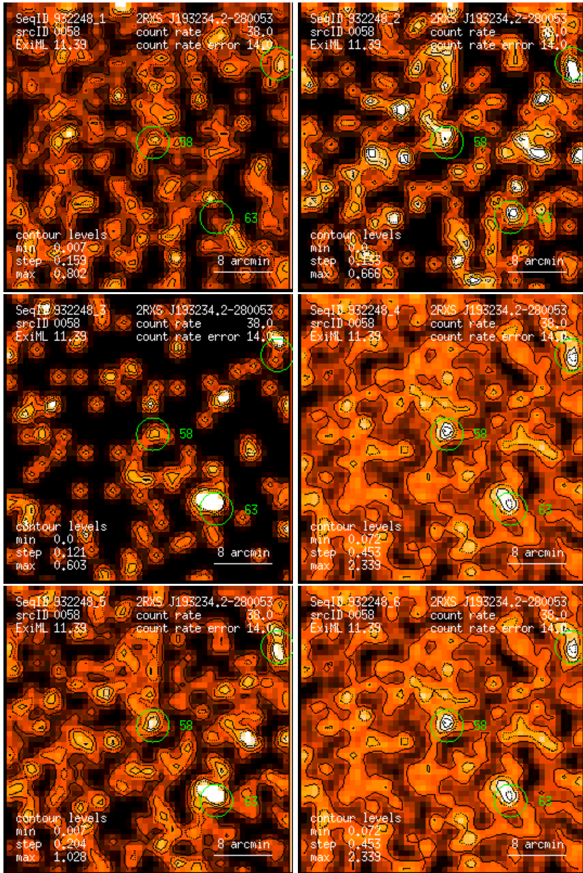
Figure 58: RASS 932248: detection 0058: band rate images, Gaussian filter: (1) PSPC channels 11 – 41, (2) 52 – 90, (3) 91 – 201, (4) 11 – 235, (5) 52 – 201, (6) 11 – 201. Broad band rates in counts/ks. Band rate contour levels in counts/ks/arcmin 2 .
