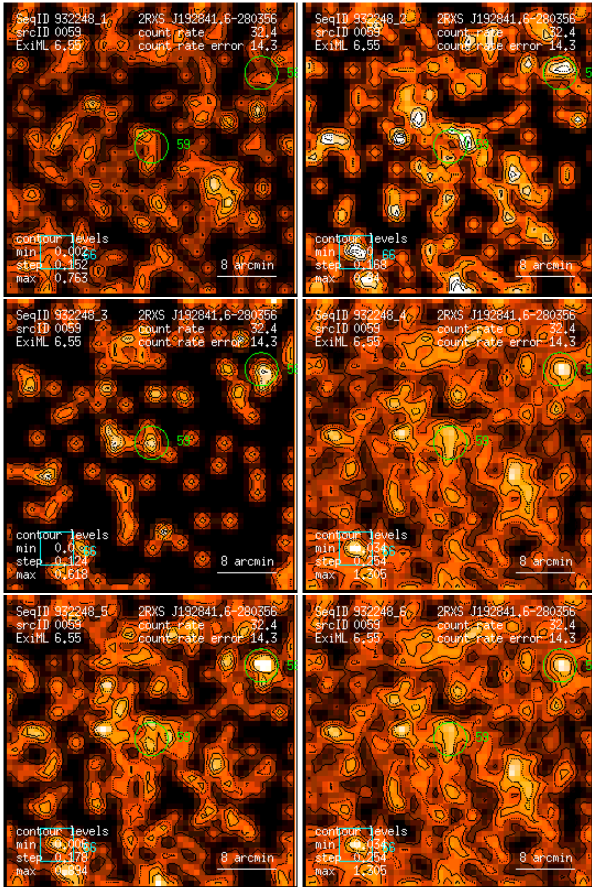
Figure 59: RASS 932248: detection 0059: band rate images, Gaussian filter: (1) PSPC channels 11 – 41, (2) 52 – 90, (3) 91 – 201, (4) 11 – 235, (5) 52 – 201, (6) 11 – 201. Broad band rates in counts/ks. Band rate contour levels in counts/ks/arcmin 2 .
