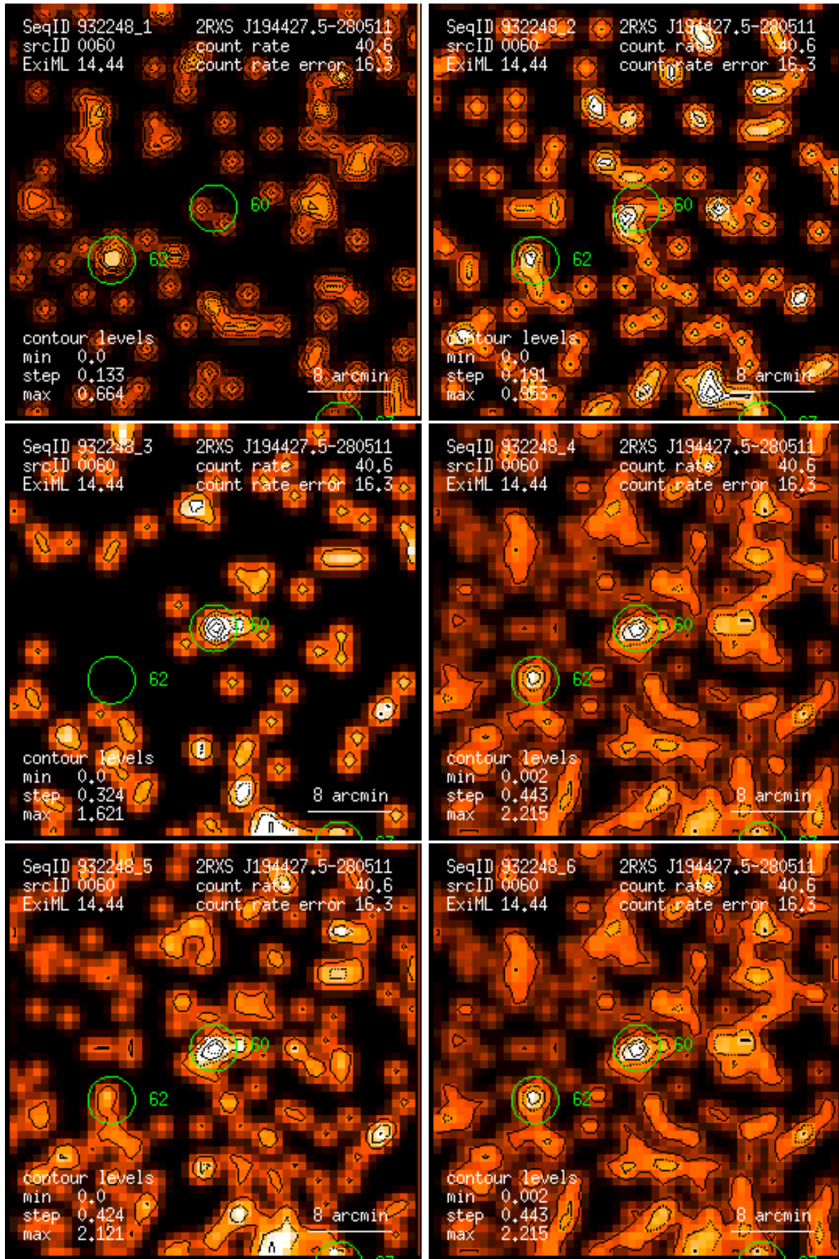
Figure 60: RASS 932248: detection 0060: band rate images, Gaussian filter: (1) PSPC channels 11 – 41, (2) 52 – 90, (3) 91 – 201, (4) 11 – 235, (5) 52 – 201, (6) 11 – 201. Broad band rates in counts/ks. Band rate contour levels in counts/ks/arcmin 2 .
