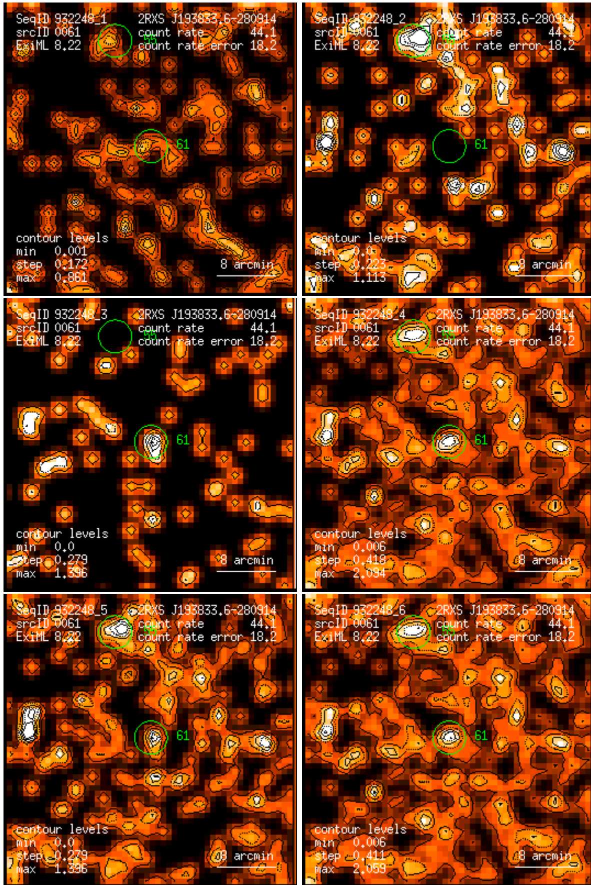
Figure 61: RASS 932248: detection 0061: band rate images, Gaussian filter: (1) PSPC channels 11 – 41, (2) 52 – 90, (3) 91 – 201, (4) 11 – 235, (5) 52 – 201, (6) 11 – 201. Broad band rates in counts/ks. Band rate contour levels in counts/ks/arcmin 2 .
