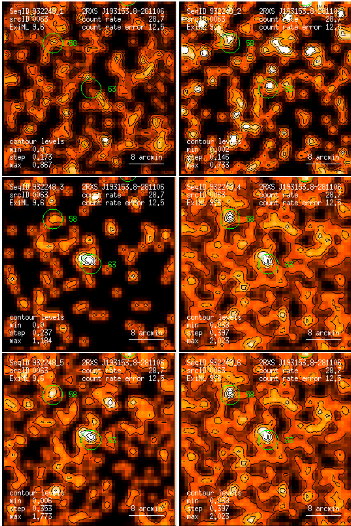
Figure 63: RASS 932248: detection 0063: band rate images, Gaussian filter: (1) PSPC channels 11 – 41, (2) 52 – 90, (3) 91 – 201, (4) 11 – 235, (5) 52 – 201, (6) 11 – 201. Broad band rates in counts/ks. Band rate contour levels in counts/ks/arcmin 2 .
