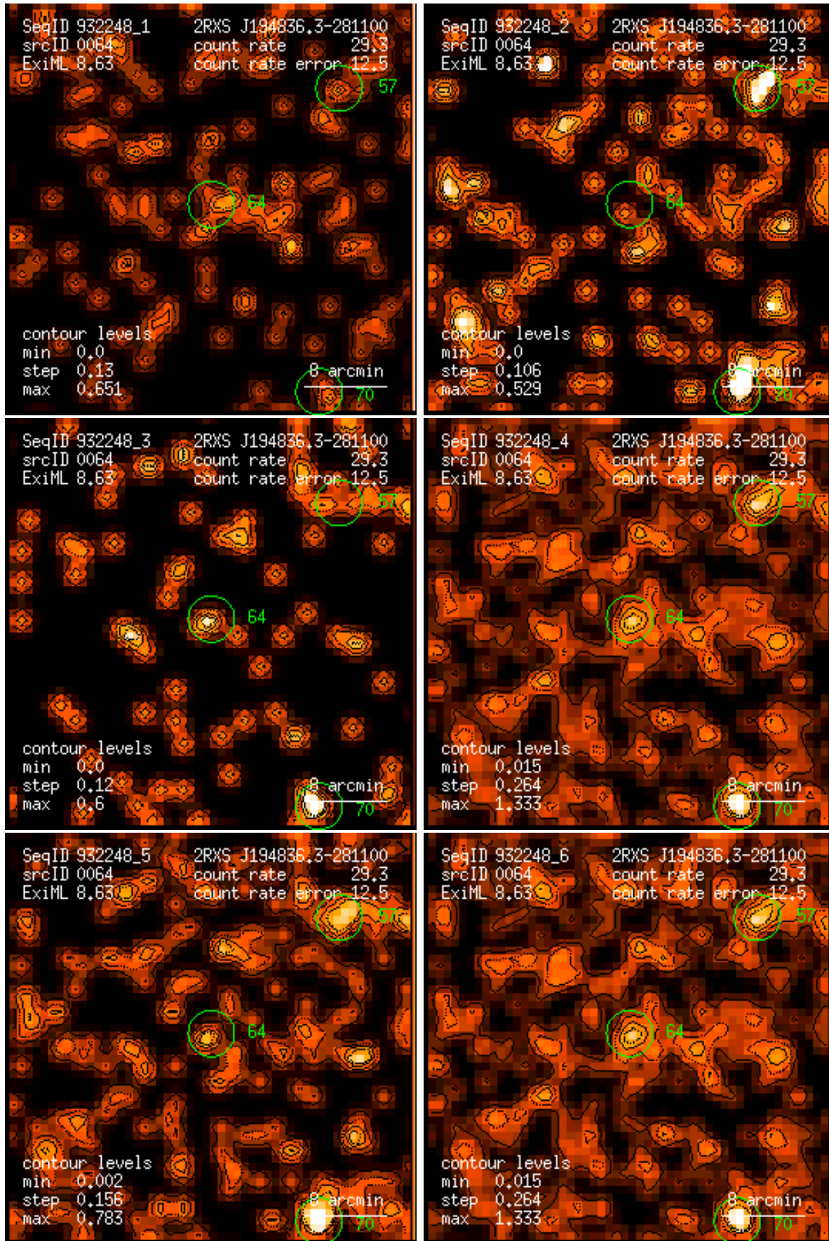
Figure 64: RASS 932248: detection 0064: band rate images, Gaussian filter: (1) PSPC channels 11 – 41, (2) 52 – 90, (3) 91 – 201, (4) 11 – 235, (5) 52 – 201, (6) 11 – 201. Broad band rates in counts/ks. Band rate contour levels in counts/ks/arcmin 2 .
