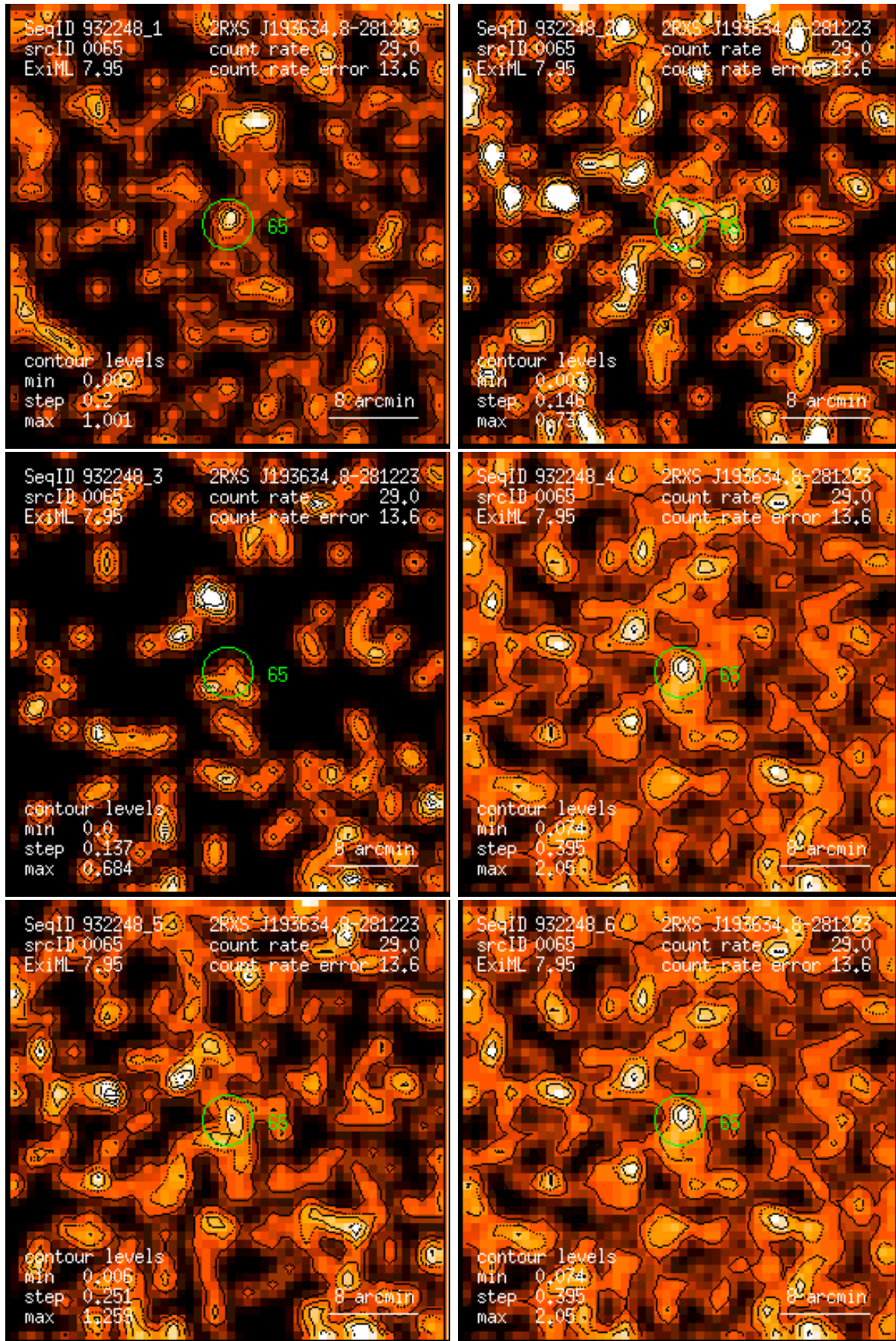
Figure 65: RASS 932248: detection 0065: band rate images, Gaussian filter: (1) PSPC channels 11 – 41, (2) 52 – 90, (3) 91 – 201, (4) 11 – 235, (5) 52 – 201, (6) 11 – 201. Broad band rates in counts/ks. Band rate contour levels in counts/ks/arcmin 2 .
